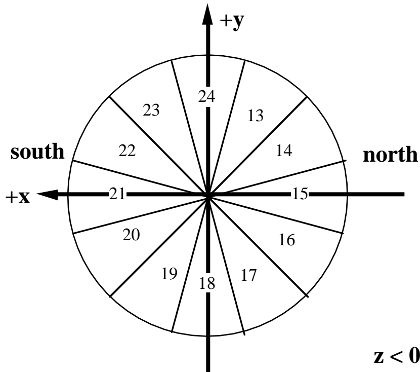
Figure 4: This is the East End view of the detector when one is looking at the endcap from the outside.
