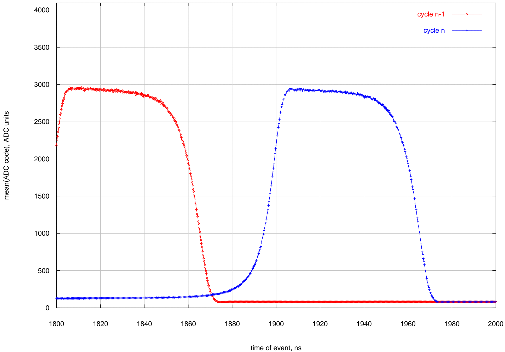
MAPMT box UV LED / WLS pulser response, trigger on two different cycles
