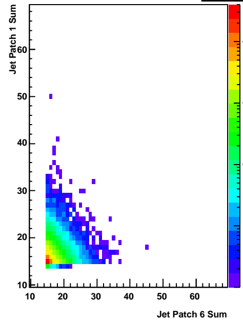
Emulated Sum Jet Patches 6 vs 1
