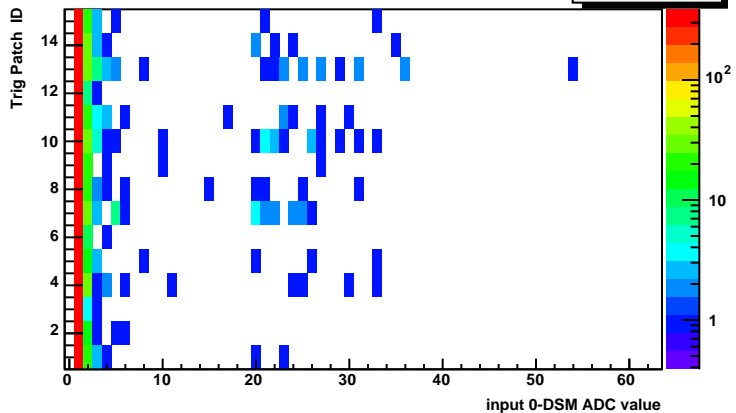
HT input, DSM layer-0, Jet Patch 5 (Steve), trig=allTrig
