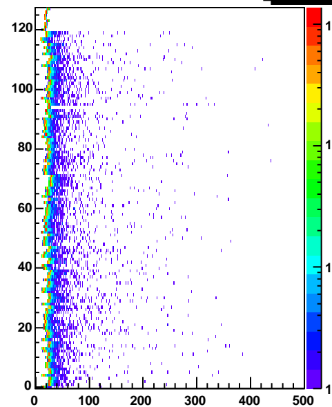
cr6 Entries 283776
