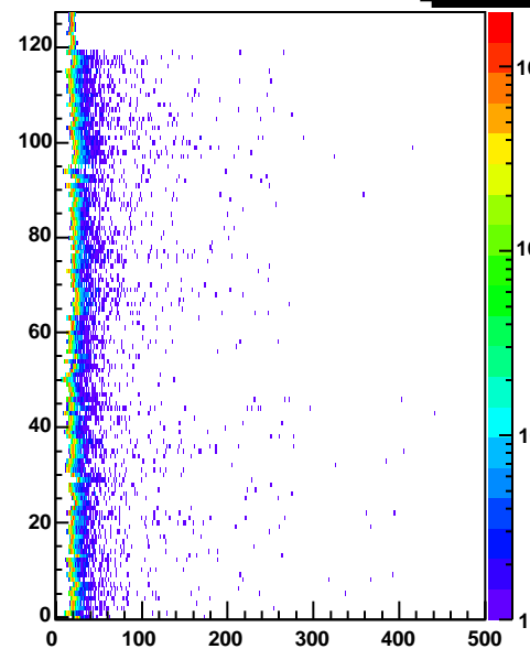
cr5 Entries 283776
