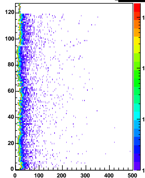
cr3 Entries 283776
