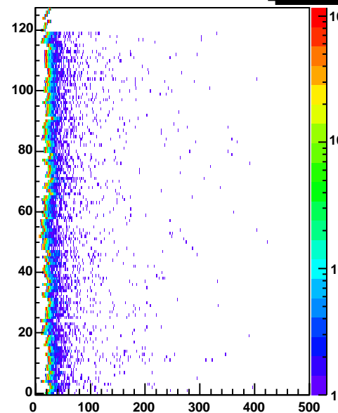
cr2 Entries 283776
