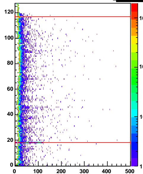
cr4 Entries 283776
