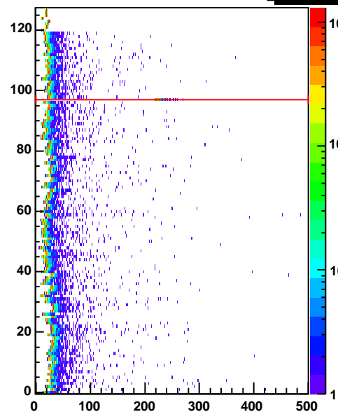
cr1 Entries 283776
