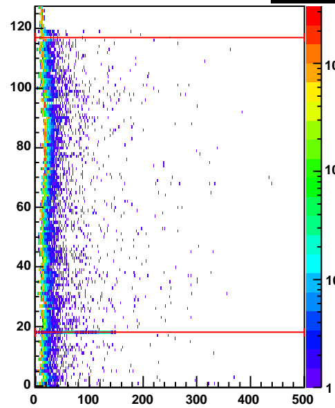
cr4 Entries 487808
