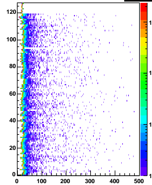
cr6 Entries 487808
