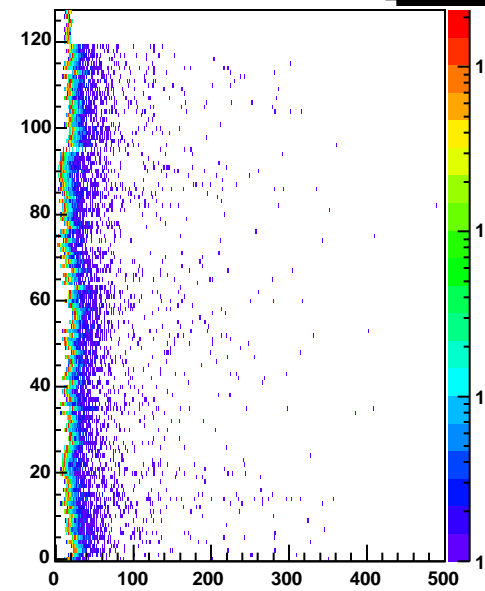
cr3 Entries 487808
