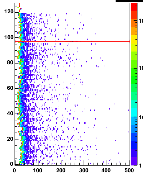
cr1 Entries 487808
