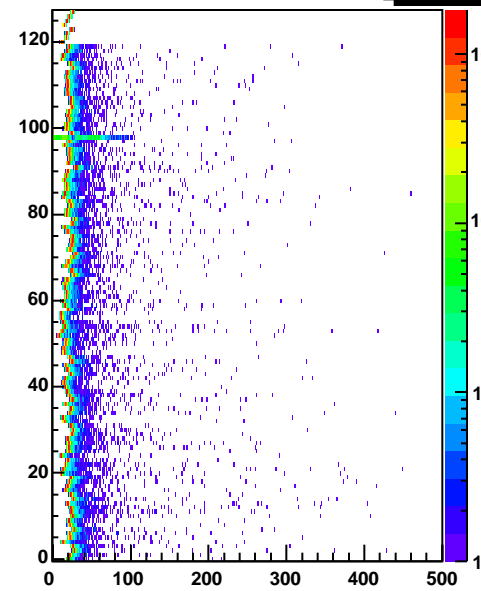
cr2 Entries 487808
