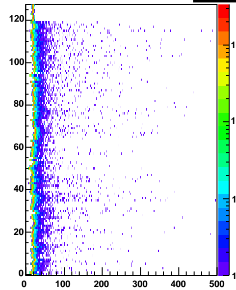
cr5 Entries 487808
