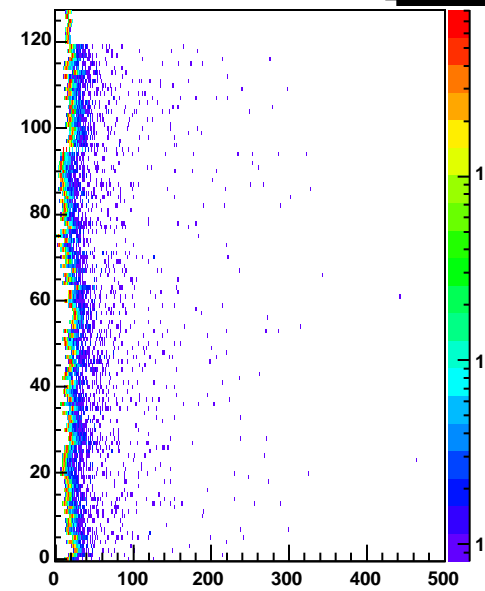
cr3 Entries 185728
