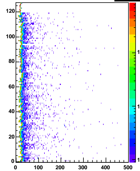
cr6 Entries 185728
