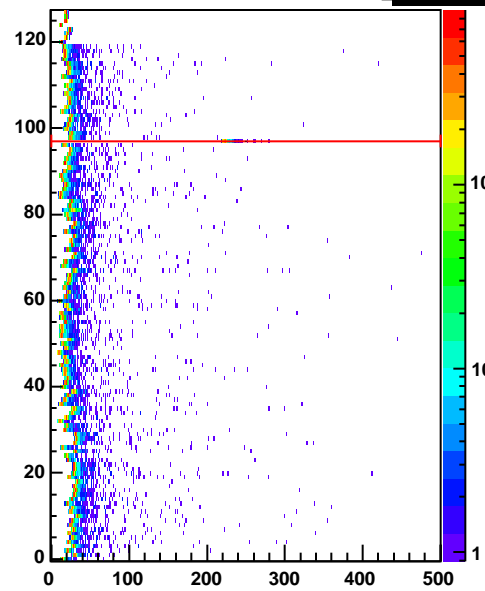
cr1 Entries 185728
