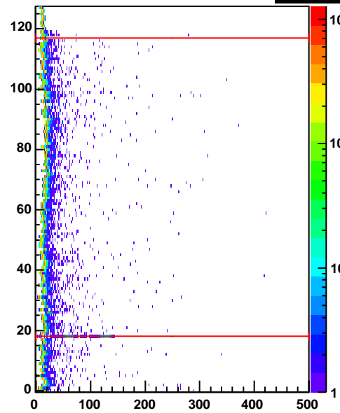
cr4 Entries 185728
