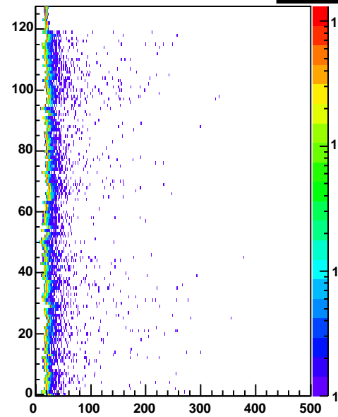
cr5 Entries 185728
