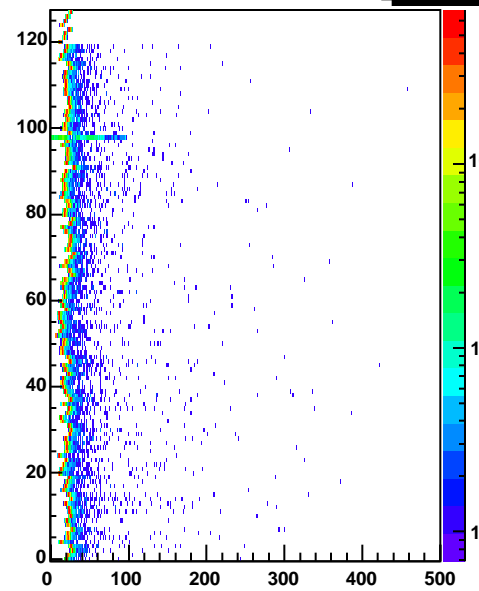
cr2 Entries 185728
