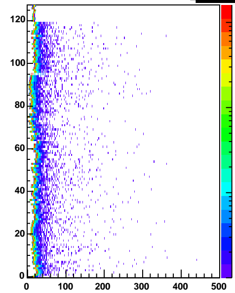
cr3 Entries 344448
