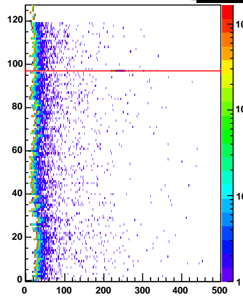
cr1 Entries 344448
