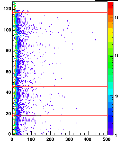
cr4 Entries 344448
