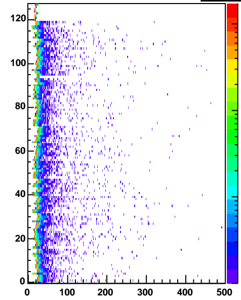
cr6 Entries 344448
