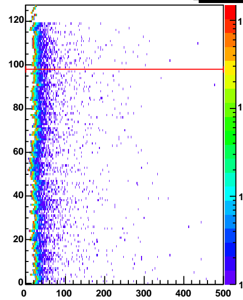
cr2 Entries 344448
