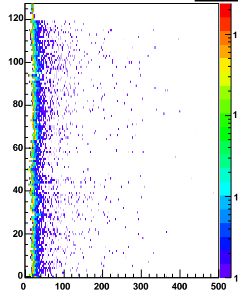
cr5 Entries 344448
