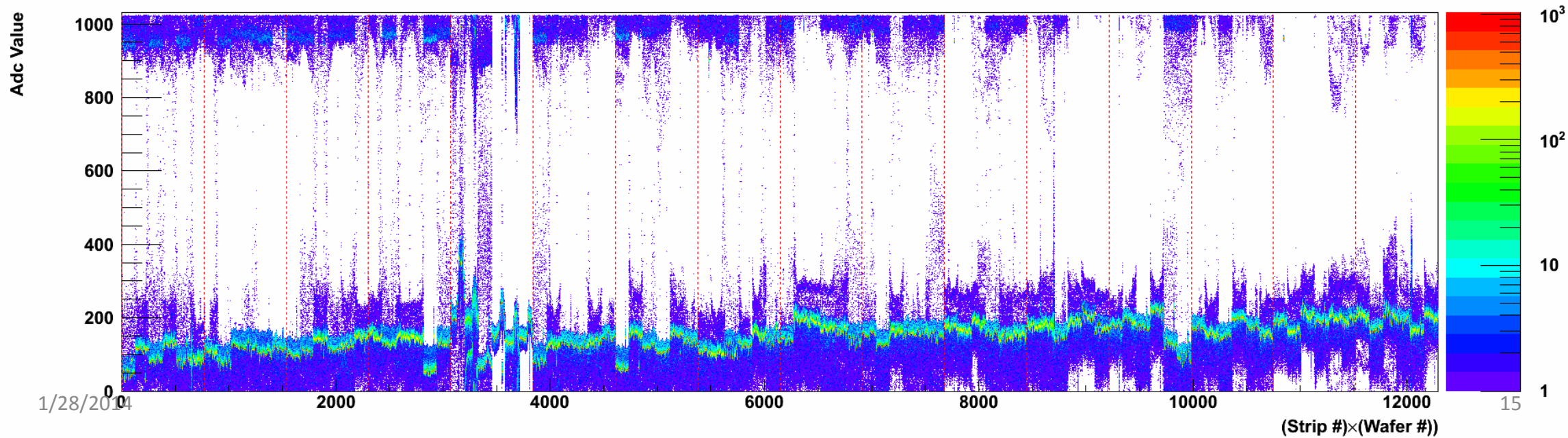
Ladder #13 N-side
