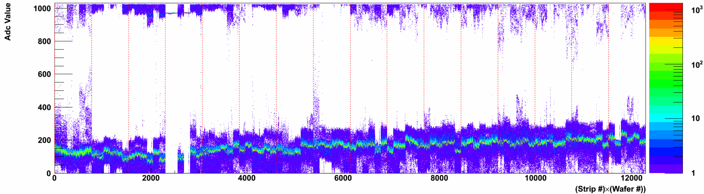
Ladder #11 N-side
