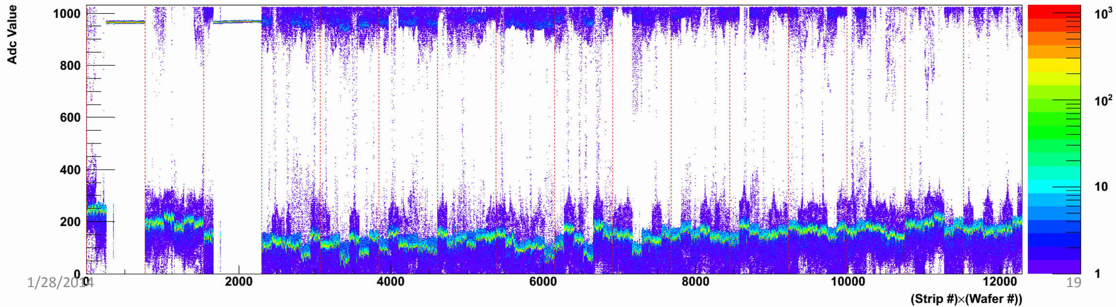
Ladder #17 N-side
