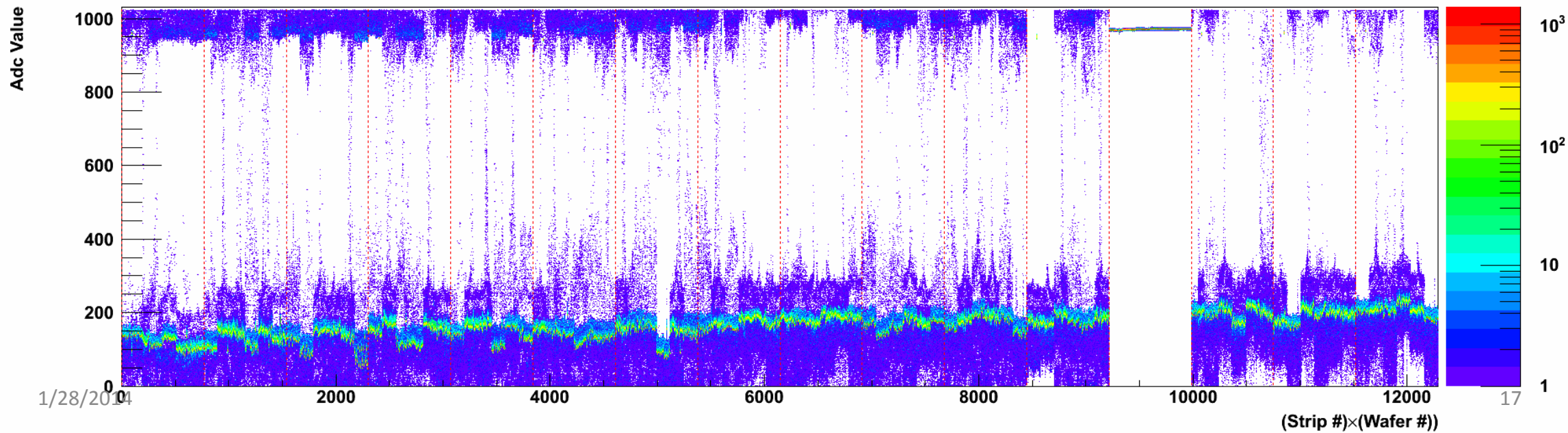
Ladder #15 N-side
