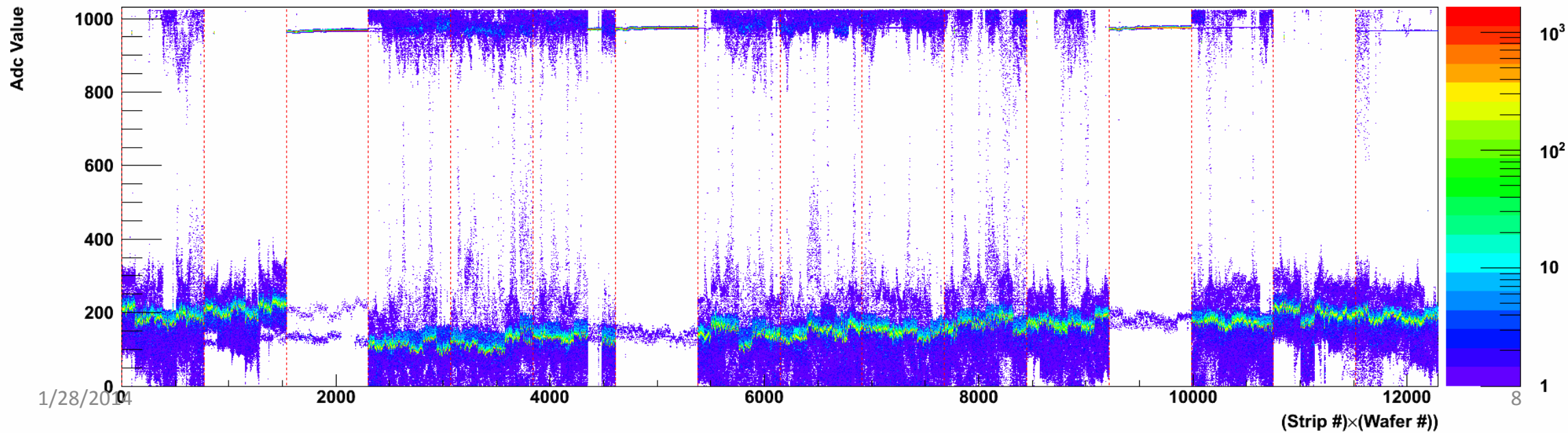
Ladder #6 N-side
