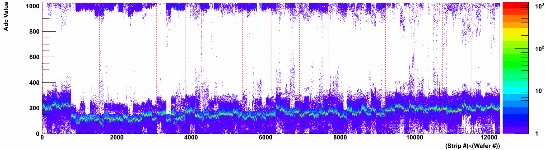
Ladder #10 N-side
