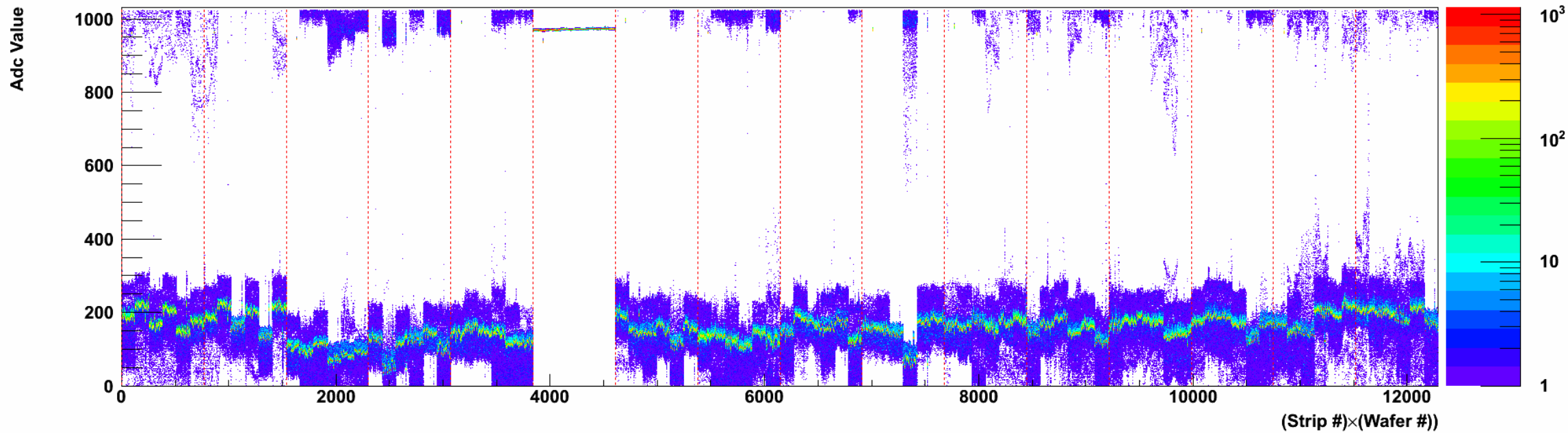
Ladder #9 N-side
