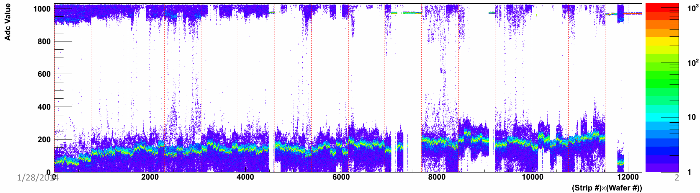
Ladder #0 N-side
