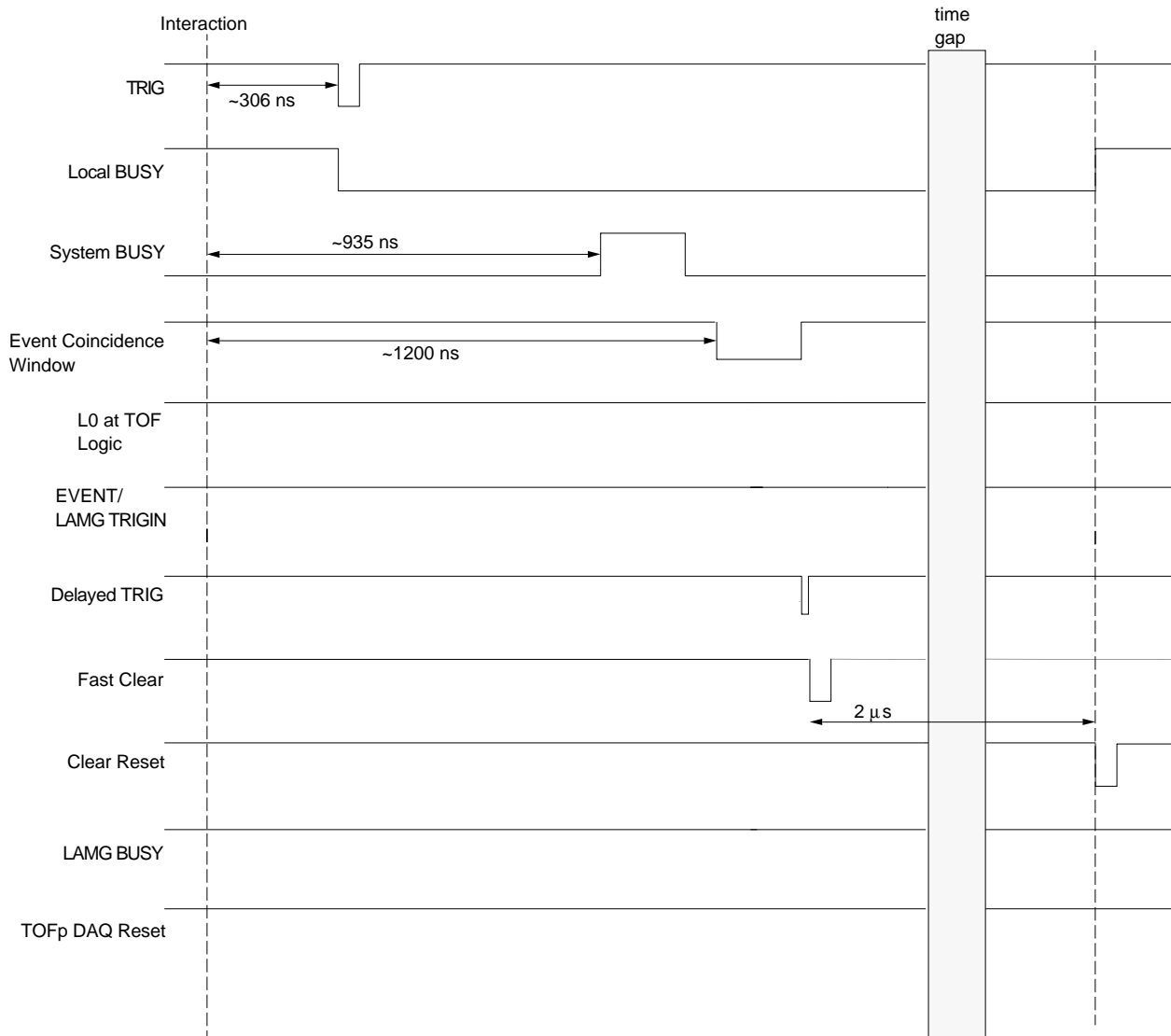
Bad Event (no L0) Timing Diagram Normal Running with 25 April 2001 Logic
