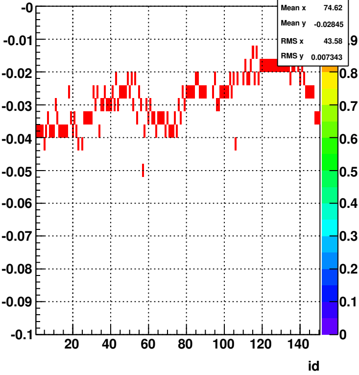
bsmdp slope vs. id (1-150)
