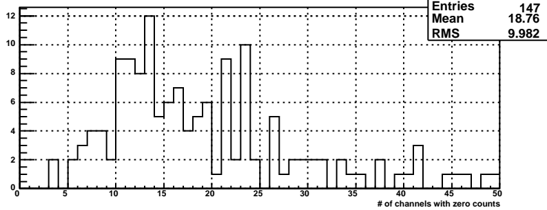
nzero for bsmde plane, mod 111
