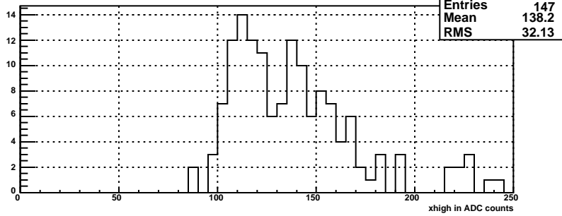
xhigh for bsmde plane, mod 111
