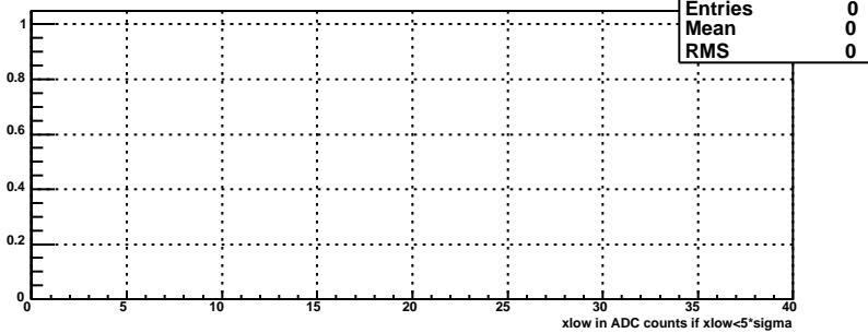
nlow for bsmde plane, mod 111
