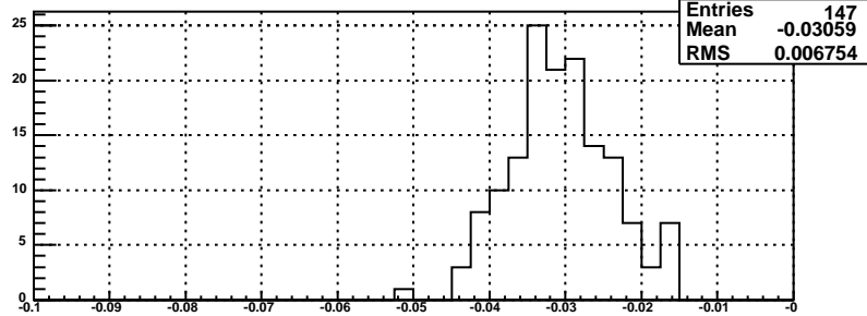
slopes for bsmde plane, mod 111
