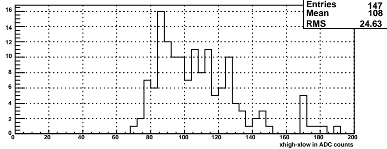
xdiff for bsmde plane, mod 111
