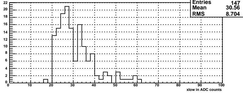
xlow for bsmde plane, mod 111
