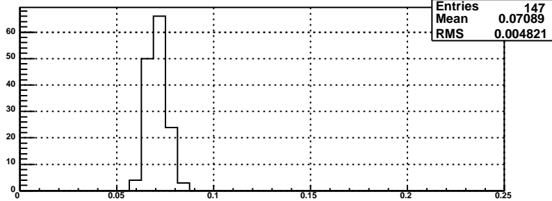
relative errors for bsmde plane, mod 111
