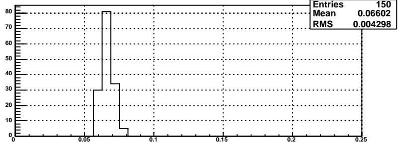
relative errors for bsm dp plane, mod 111
