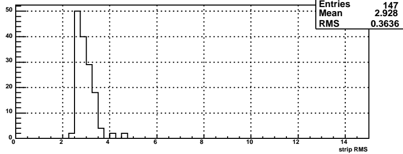
rms for bsmde plane, mod 111
