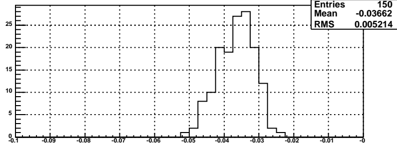
slopes for bsm dp plane, mod 111
