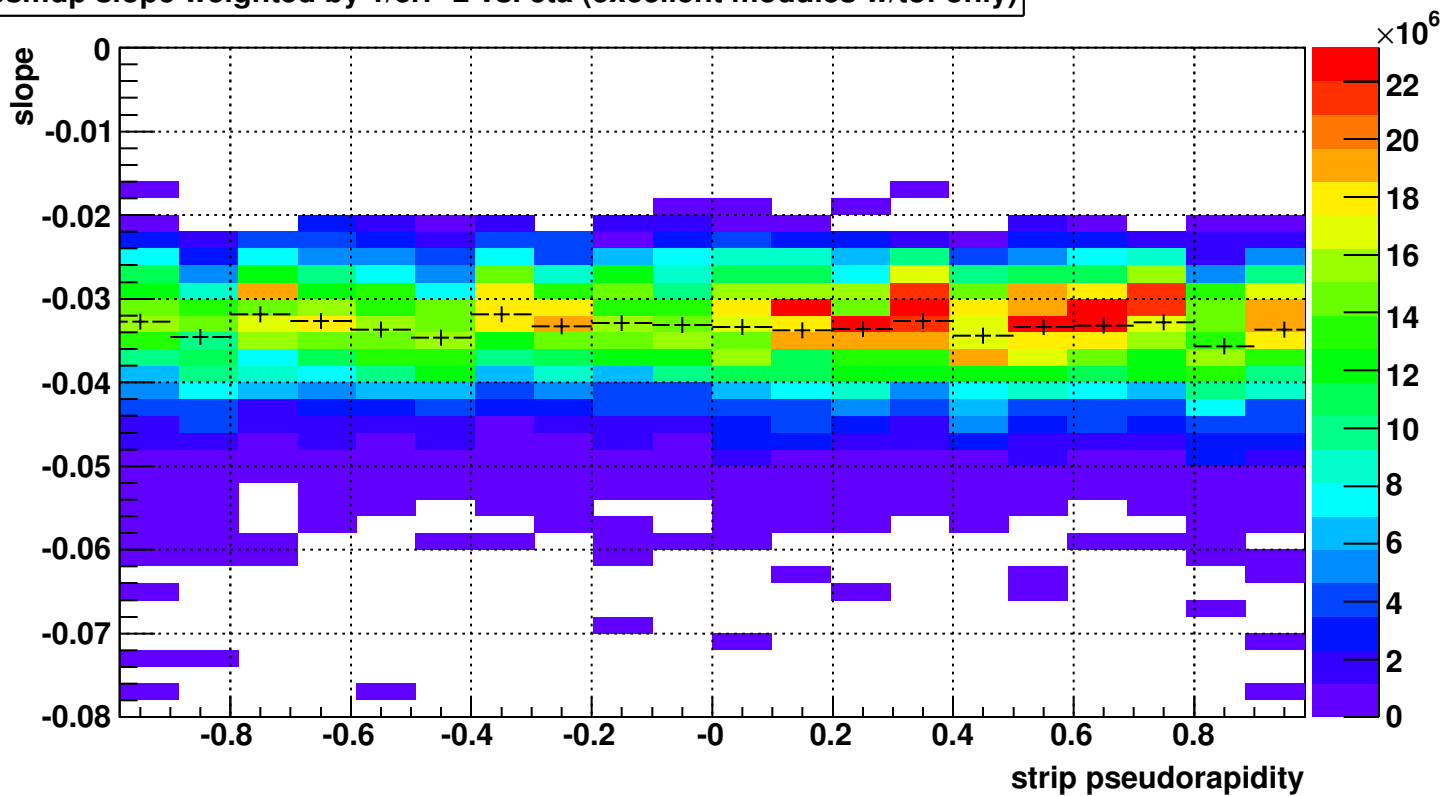
bsmdp slope weighted by 1/\text{err}^2 vs. eta (excellent modules w/tof only)
