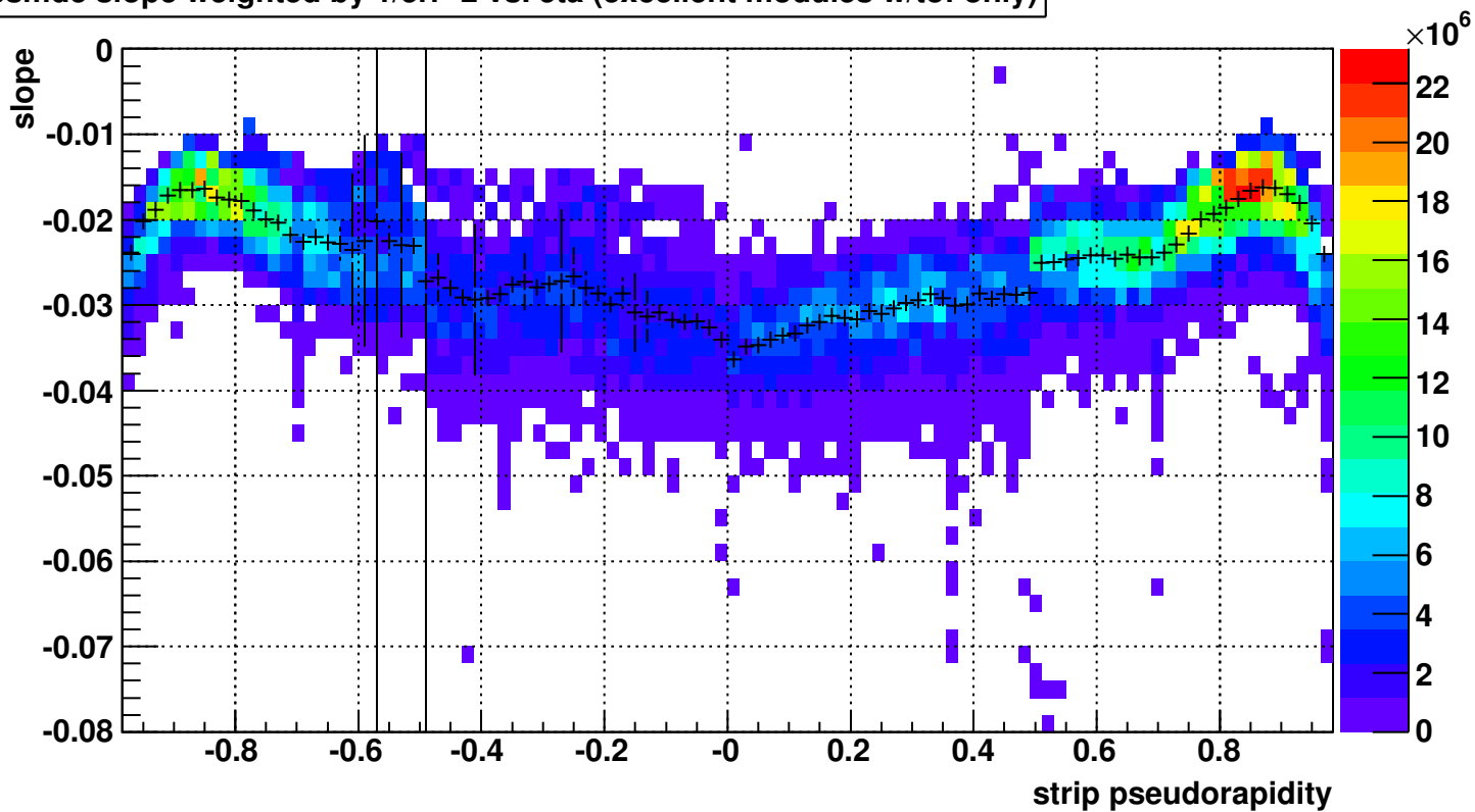
bsmde slope weighted by 1/\text{err}^2 vs. eta (excellent modules w/tof only)
