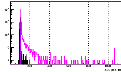
BSMD Strip 462_e
