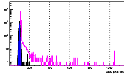
BSMD Strip 956_e
