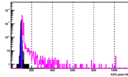
BSMD Strip 1512_p
