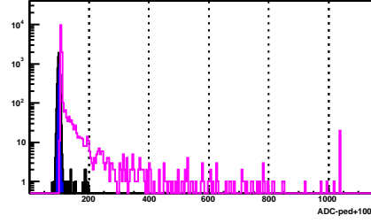
BSMD Strip 686_e
