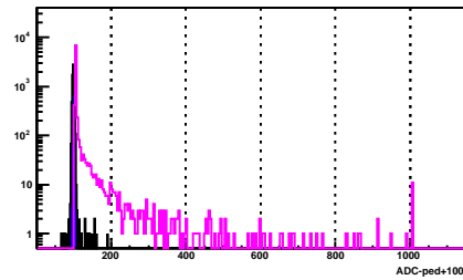
BSMD Strip 1061_p
