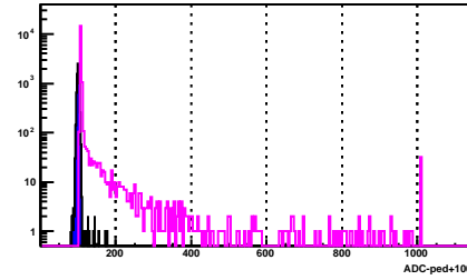
BSMD Strip 132_e
