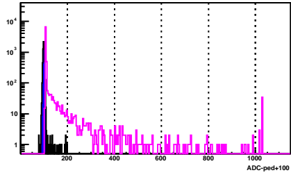
BSMD Strip 1030_e
