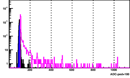
BSMD Strip 1417_p
