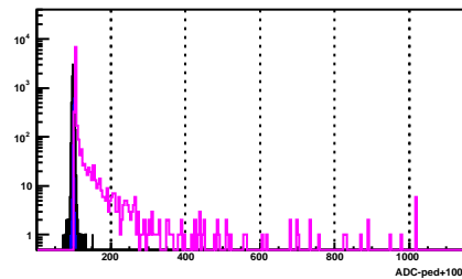
BSMD Strip 1994_p
