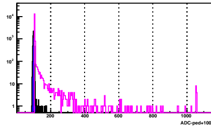
BSMD Strip 485_e
