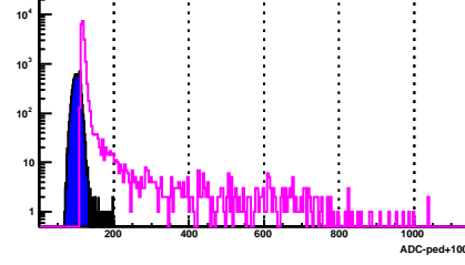
BSMD Strip 1493_e
