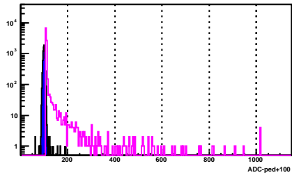
BSMD Strip 154_p
