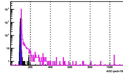
BSMD Strip 654_e
