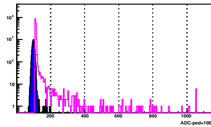
BSMD Strip 755_e
