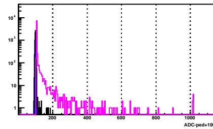
BSMD Strip 1086_e
