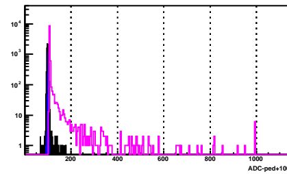
BSMD Strip 2076_p
