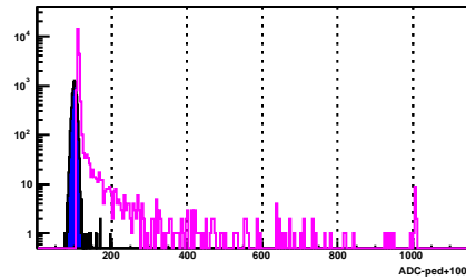
BSMD Strip 1286_e
