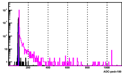
BSMD Strip 469_p
