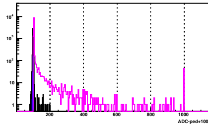
BSMD Strip 1169_e
