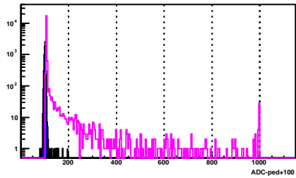
BSMD Strip 409_e
