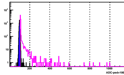
BSMD Strip 1478_p
