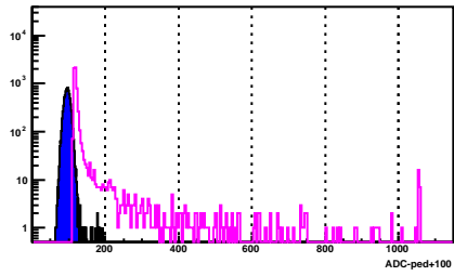
BSMD Strip 529_e
