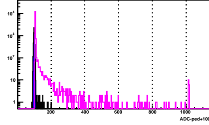
BSMD Strip 113_e
