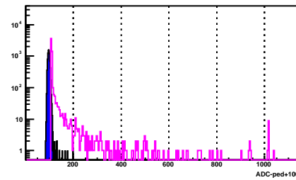
BSMD Strip 306_e
