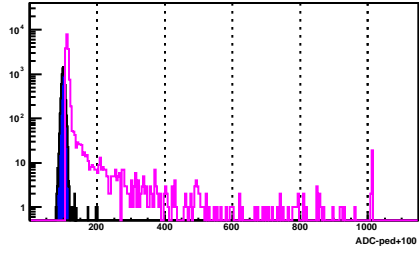
BSMD Strip 2065_e
