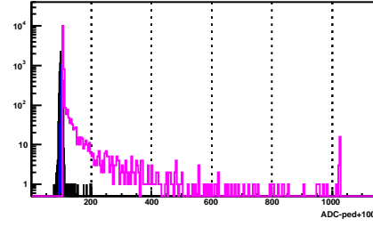
BSMD Strip 263_e
