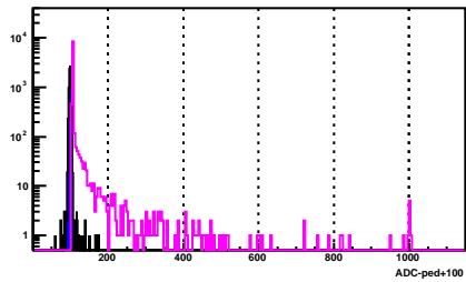
BSMD Strip 1057_p
