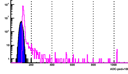
BSMD Strip 1556_e
