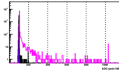
BSMD Strip 1115_e
