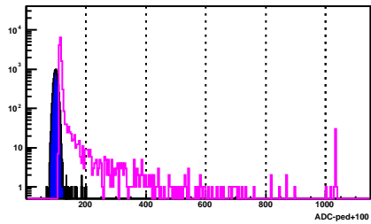
BSMD Strip 250_e
