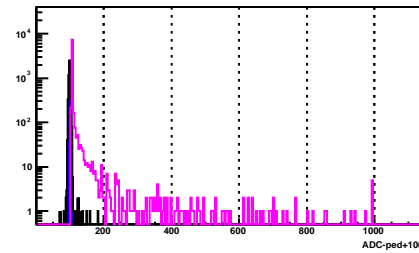
BSMD Strip 1707_p
