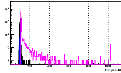
BSMD Strip 1710_e
