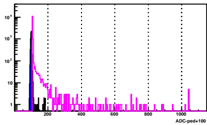
BSMD Strip 634_e
