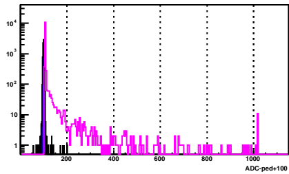
BSMD Strip 1900_p
