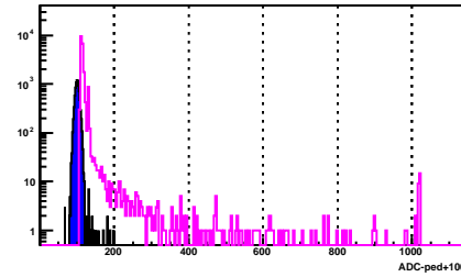
BSMD Strip 2040_e
