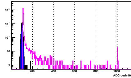
BSMD Strip 1284_e
