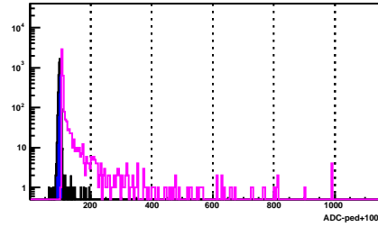
BSMD Strip 2201_p
