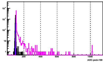
BSMD Strip 1957_p
