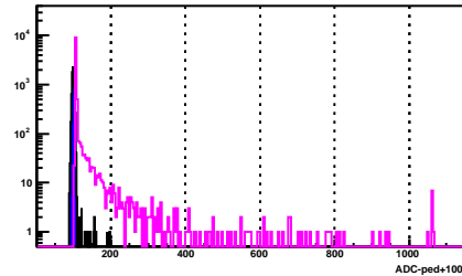
BSMD Strip 473_e
