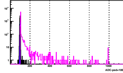
BSMD Strip 1724_p
