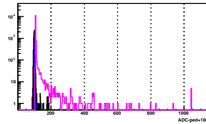
BSMD Strip 642_e
