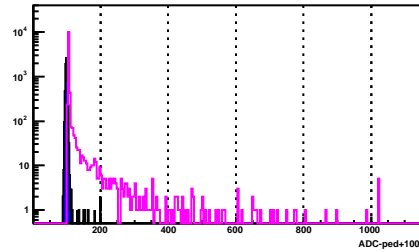
BSMD Strip 1058_e
