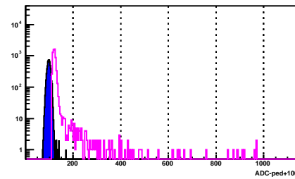
BSMD Strip 2226_p
