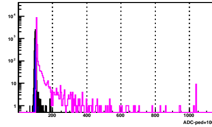
BSMD Strip 465_p
