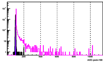
BSMD Strip 1858_p
