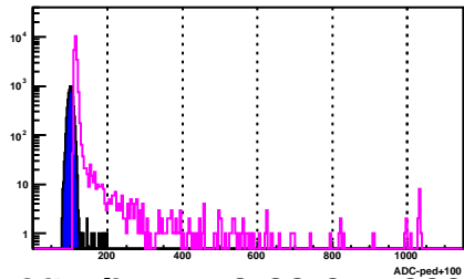
BSMD Strip 2008_e
