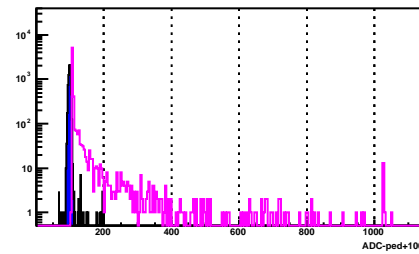
BSMD Strip 1461_p
