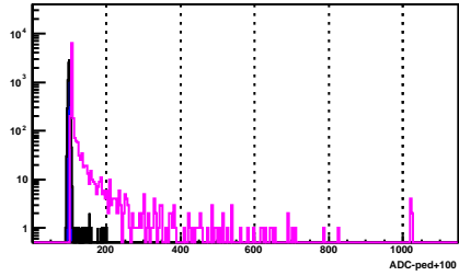
BSMD Strip 1075_e
