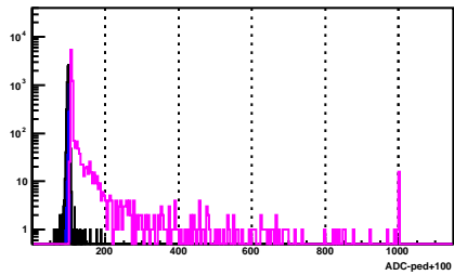
BSMD Strip 1582_p
