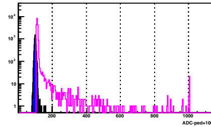
BSMD Strip 2076_e
