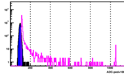
BSMD Strip 536_e
