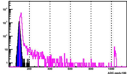
BSMD Strip 1942_e
