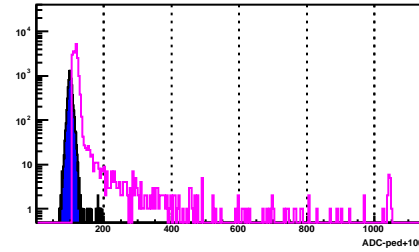
BSMD Strip 1905_e
