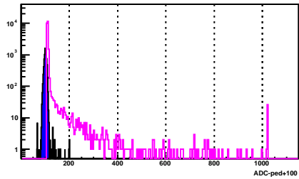
BSMD Strip 880_e
