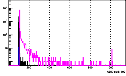
BSMD Strip 1102_e
