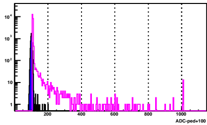
BSMD Strip 1300_e
