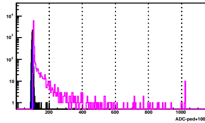
BSMD Strip 1685_e
