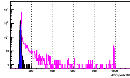
BSMD Strip 419_e
