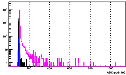
BSMD Strip 649_e
