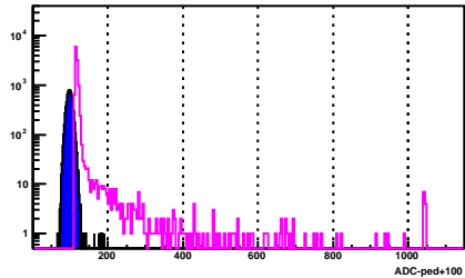
BSMD Strip 217_e
