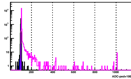
BSMD Strip 1943_p
