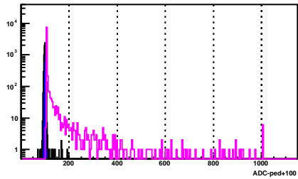
BSMD Strip 694_p
