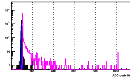
BSMD Strip 876_p
