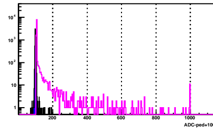
BSMD Strip 1119_p
