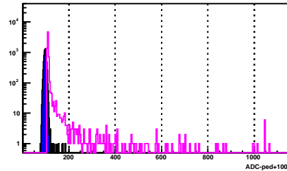
BSMD Strip 1373_p
