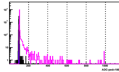
BSMD Strip 1736_p
