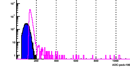
BSMD Strip 1529_e Channel 1529 has bad status 21
