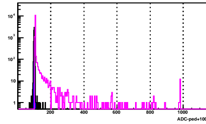
BSMD Strip 1167_p
