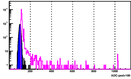
BSMD Strip 2002_e
