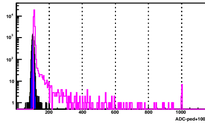
BSMD Strip 1040_p
