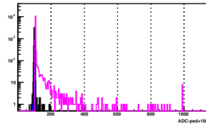
BSMD Strip 1254_p
