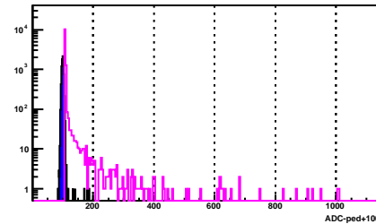
BSMD Strip 660_e
