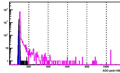
BSMD Strip 1856_e
