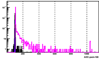
BSMD Strip 502_p
