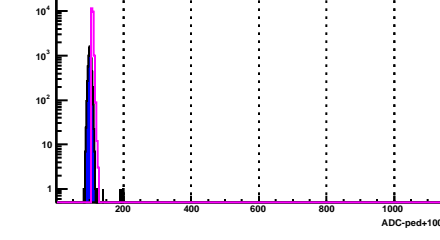
BSMD Strip 953_p Channel 953 has bad status 448
