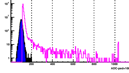
BSMD Strip 1496_e Channel 1496 has bad status 448
