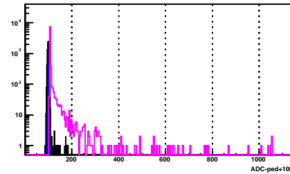
BSMD Strip 627_e
