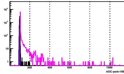
BSMD Strip 1073_e
