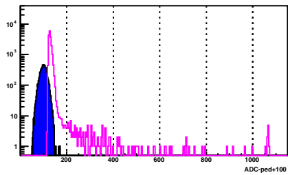
BSMD Strip 904_e
