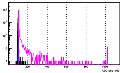
BSMD Strip 1879_p
