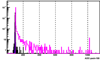
BSMD Strip 1912_p
