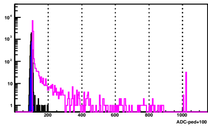
BSMD Strip 1729_e
