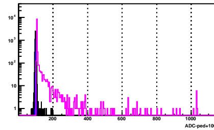
BSMD Strip 1839_p
