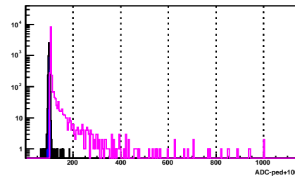
BSMD Strip 1056_p
