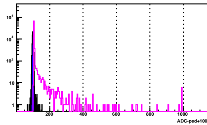
BSMD Strip 1694_p
