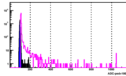
BSMD Strip 1859_e
