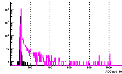
BSMD Strip 1932_p
