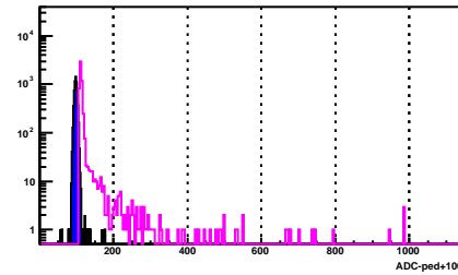
BSMD Strip 2196_p
