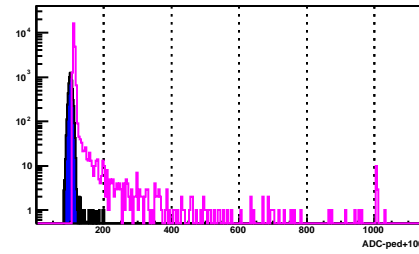
BSMD Strip 1272_e
