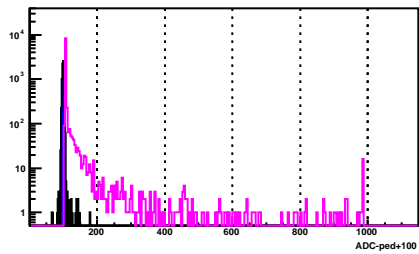
BSMD Strip 1279_p
