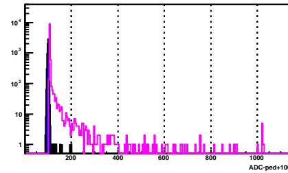
BSMD Strip 1056_e
