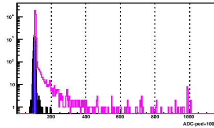
BSMD Strip 359_p
