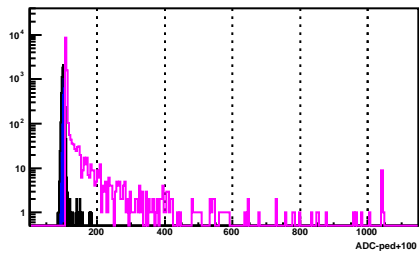
BSMD Strip 199_e
