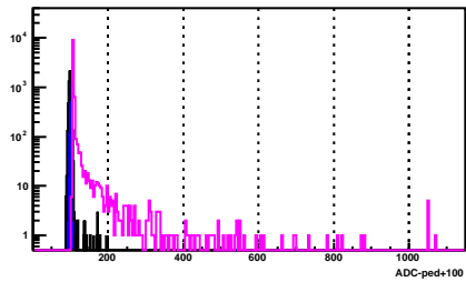
BSMD Strip 637_e
