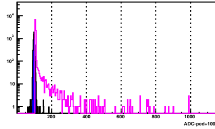
BSMD Strip 746_p
