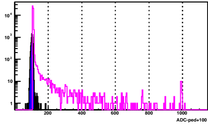
BSMD Strip 400_p
