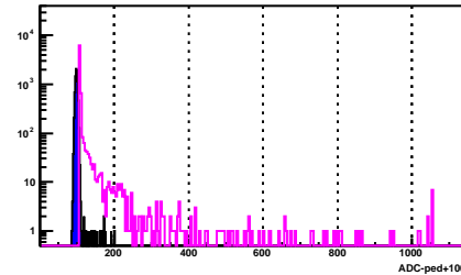
BSMD Strip 924_e
