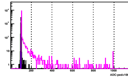
BSMD Strip 1139_p
