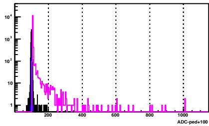
BSMD Strip 1927_p
