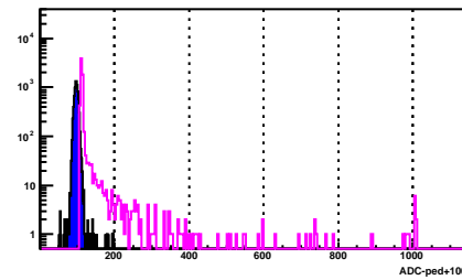
BSMD Strip 1506_p
