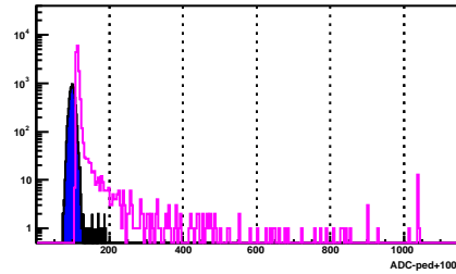
BSMD Strip 968_e
