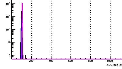
BSMD Strip 564_p Channel 564 has bad status 448
