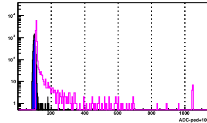
BSMD Strip 954_e
