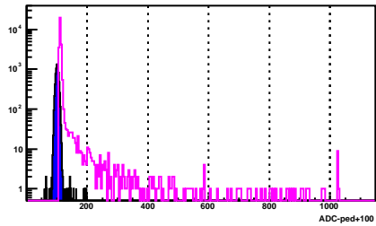
BSMD Strip 919_p
