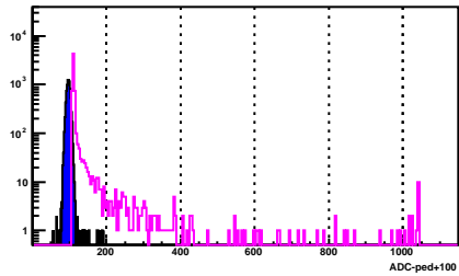
BSMD Strip 1369_p
