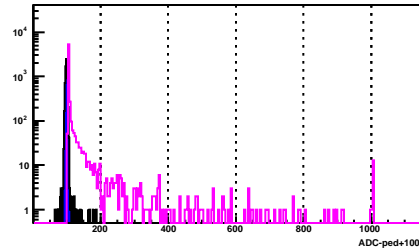
BSMD Strip 689_p
