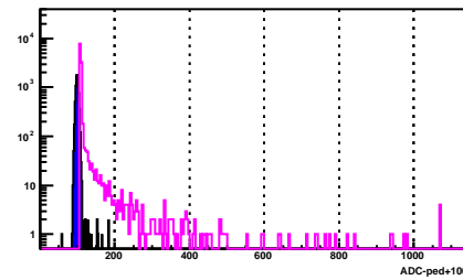
BSMD Strip 1356_e
