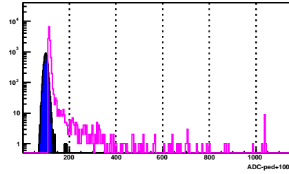
BSMD Strip 971_e
