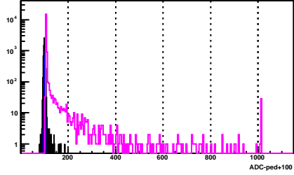
BSMD Strip 118_e
