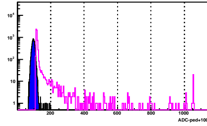
BSMD Strip 533_e
