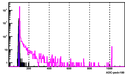
BSMD Strip 724_e
