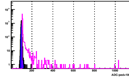
BSMD Strip 777_p
