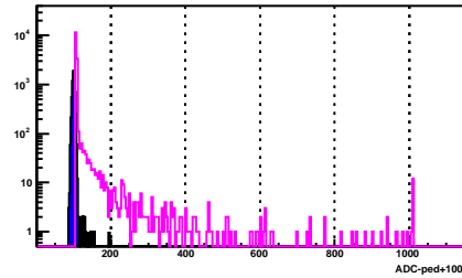
BSMD Strip 1748_e
