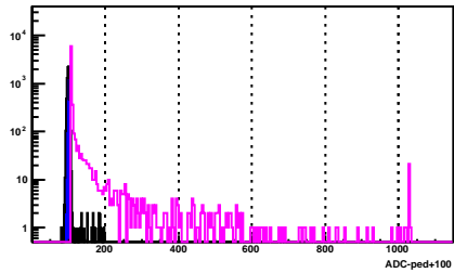
BSMD Strip 1015_e
