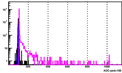
BSMD Strip 1609_e
