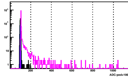
BSMD Strip 626_e
