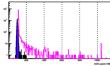
BSMD Strip 203_e
