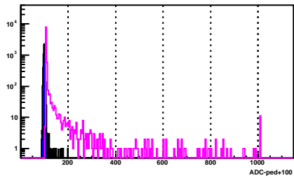
BSMD Strip 1702_e
