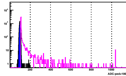
BSMD Strip 761_p
