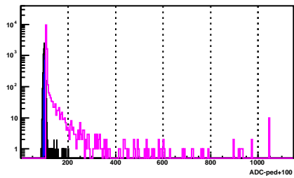
BSMD Strip 1849_e
