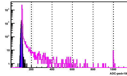
BSMD Strip 360_p
