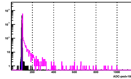
BSMD Strip 1077_p
