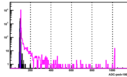
BSMD Strip 1253_e
