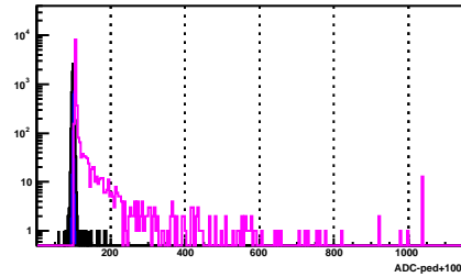
BSMD Strip 1808_p
