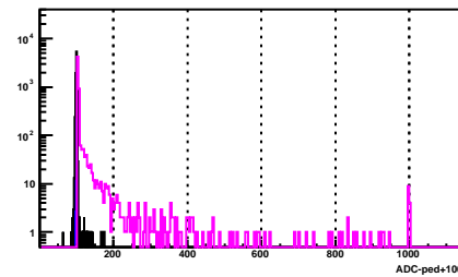
BSMD Strip 1110_p
