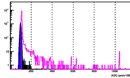
BSMD Strip 845_e
