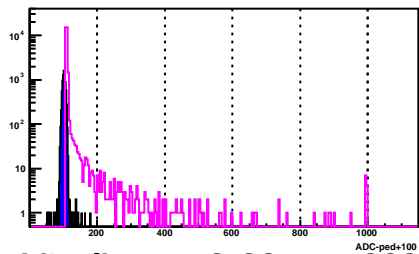
BSMD Strip 343_p
