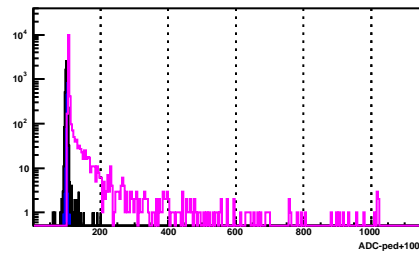
BSMD Strip 1880_p
