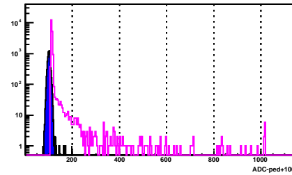
BSMD Strip 1287_e
