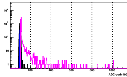
BSMD Strip 2111_p
