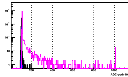
BSMD Strip 1140_e
