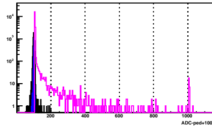
BSMD Strip 1616_e
