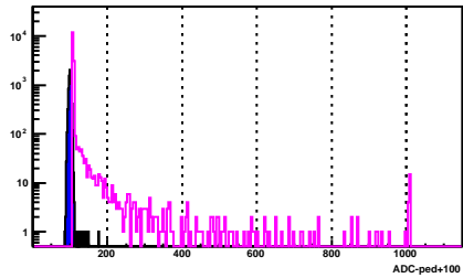
BSMD Strip 1750_e
