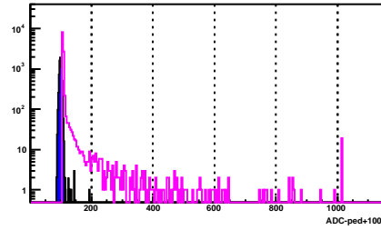
BSMD Strip 1709_e
