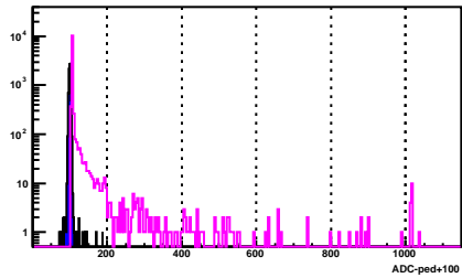
BSMD Strip 1909_p
