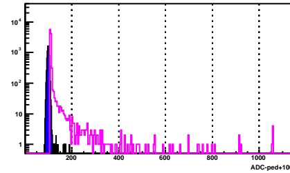
BSMD Strip 1806_e
