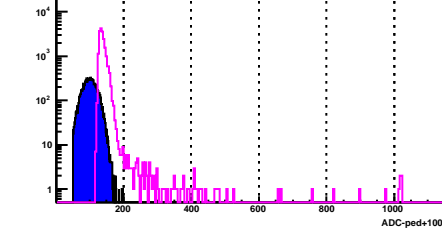
BSMD Strip 1526_e Channel 1526 has bad status 21
