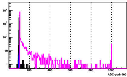
BSMD Strip 1195_e
