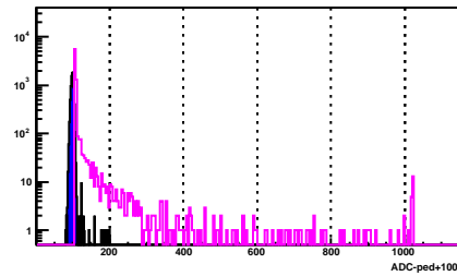
BSMD Strip 1481_p
