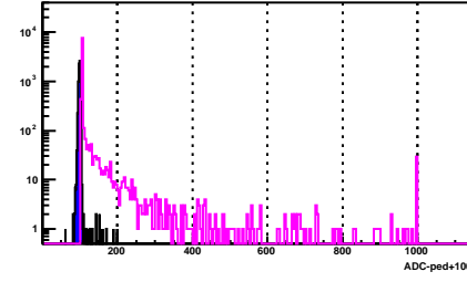
BSMD Strip 429_e
