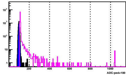
BSMD Strip 955_e
