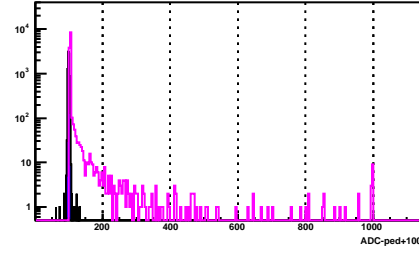
BSMD Strip 1133_p
