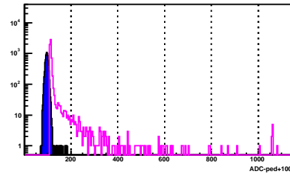
BSMD Strip 515_e
