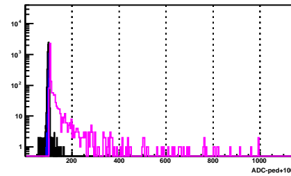
BSMD Strip 1584_p
