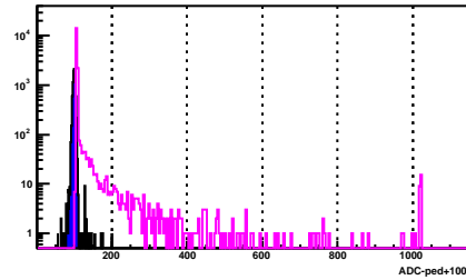
BSMD Strip 1613_e
