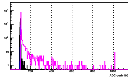
BSMD Strip 1220_e
