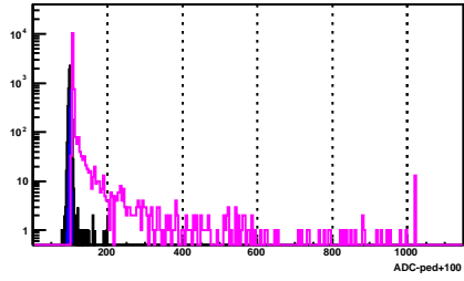
BSMD Strip 265_e
