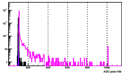
BSMD Strip 1138_e
