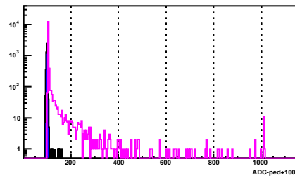
BSMD Strip 1250_e
