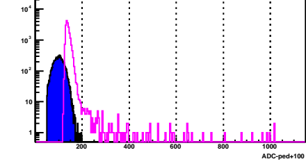
BSMD Strip 1522_e Channel 1522 has bad status 21
