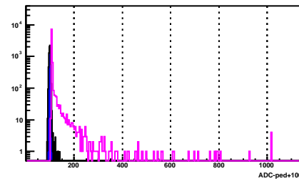
BSMD Strip 1206_e
