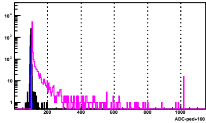
BSMD Strip 682_p
