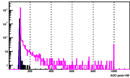
BSMD Strip 1768_e
