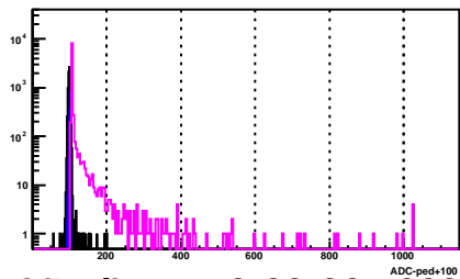
BSMD Strip 1843_p
