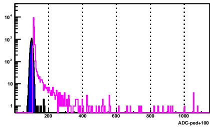
BSMD Strip 757_e
