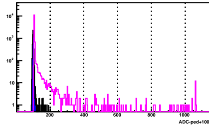
BSMD Strip 488_e
