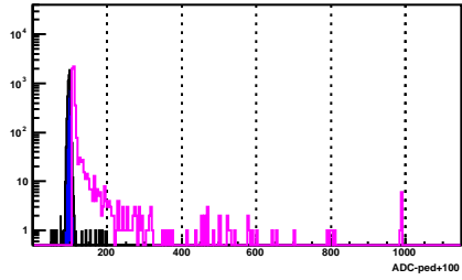
BSMD Strip 2197_p
