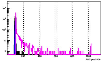
BSMD Strip 307_e
