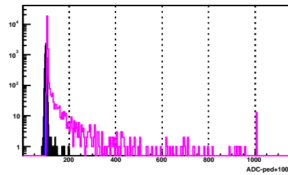
BSMD Strip 1304_e
