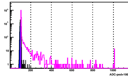
BSMD Strip 1736_e
