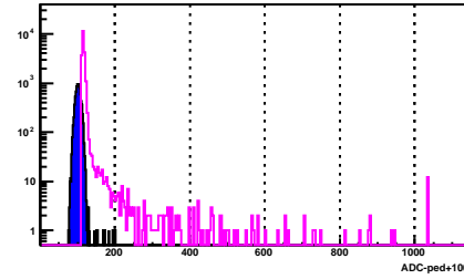
BSMD Strip 2007_e
