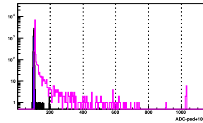
BSMD Strip 1089_e
