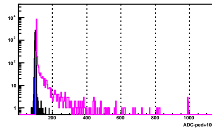
BSMD Strip 1116_p
