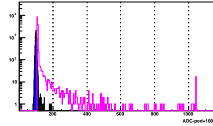
BSMD Strip 597_e
