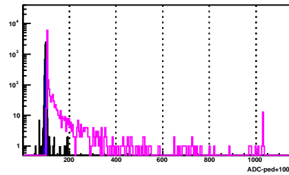
BSMD Strip 1463_p
