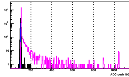
BSMD Strip 566_e
