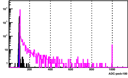
BSMD Strip 427_e
