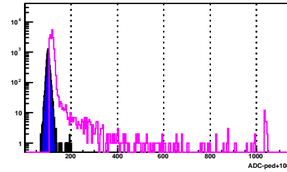
BSMD Strip 1920_e
