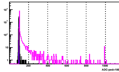
BSMD Strip 1271_p
