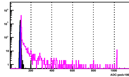
BSMD Strip 311_e
