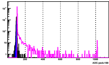
BSMD Strip 1615_e
