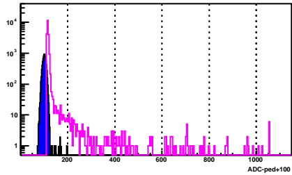
BSMD Strip 157_e
