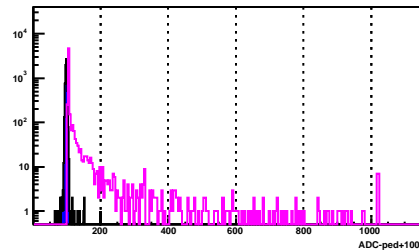
BSMD Strip 1991_p
