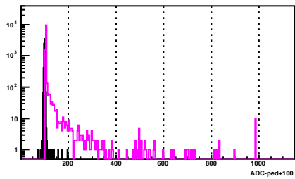
BSMD Strip 1744_p
