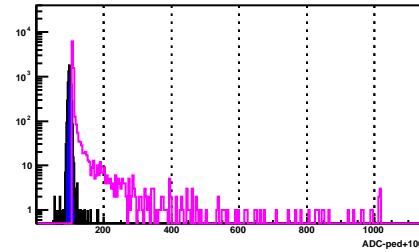
BSMD Strip 879_p
