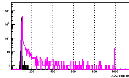
BSMD Strip 1740_p
