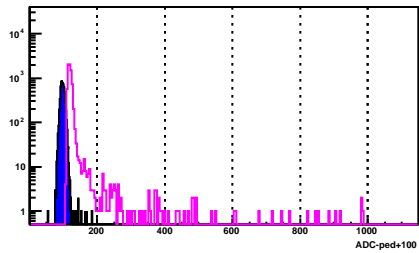
BSMD Strip 2215_p
