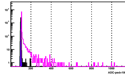
BSMD Strip 1071_e
