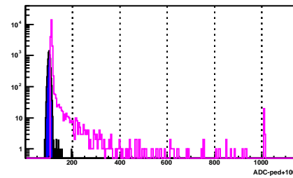
BSMD Strip 1296_e
