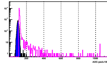
BSMD Strip 156_e
