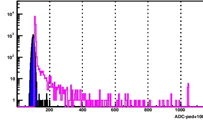
BSMD Strip 833_e
