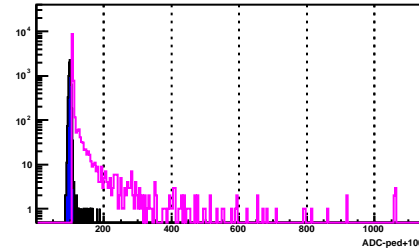
BSMD Strip 495_e
