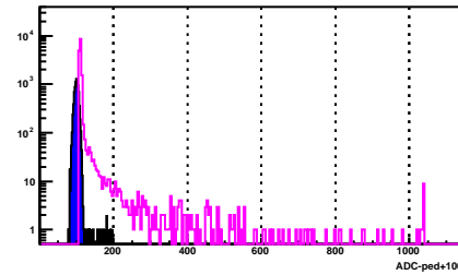
BSMD Strip 846_e
