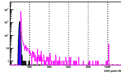
BSMD Strip 749_e
