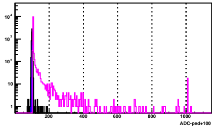
BSMD Strip 250_p
