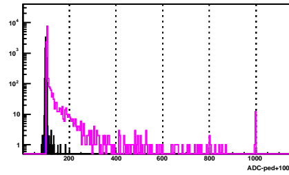
BSMD Strip 1121_p
