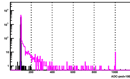
BSMD Strip 1103_p
