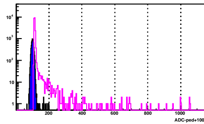
BSMD Strip 1415_e
