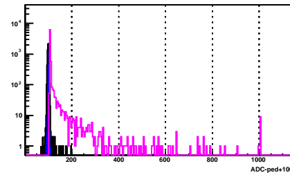
BSMD Strip 1662_p
