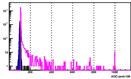
BSMD Strip 334_p
