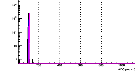
BSMD Strip 231_p
