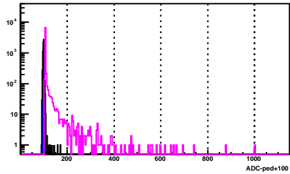
BSMD Strip 1072_e
