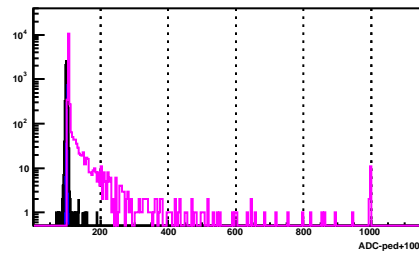
BSMD Strip 1115_p
