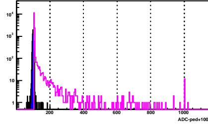
BSMD Strip 269_p
