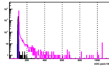
BSMD Strip 501_e
