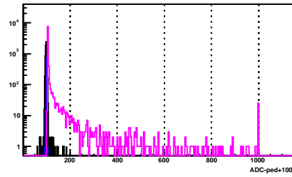
BSMD Strip 2081_p
