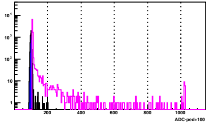
BSMD Strip 1717_e
