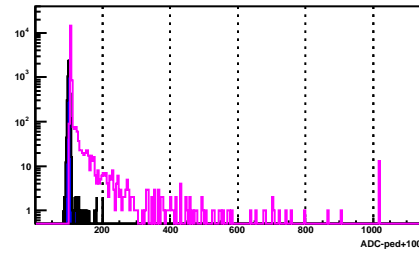
BSMD Strip 110_e
