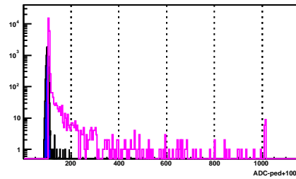
BSMD Strip 1256_e
