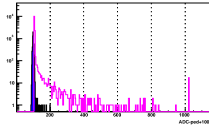
BSMD Strip 1751_e
