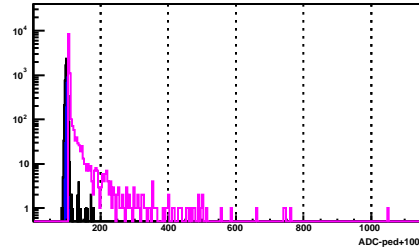
BSMD Strip 1826_e
