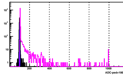
BSMD Strip 143_p
