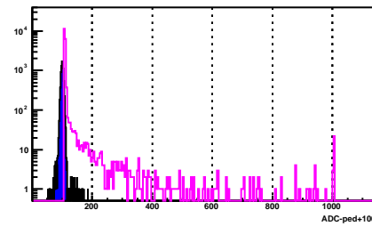
BSMD Strip 1626_e
