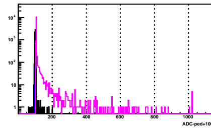
BSMD Strip 1896_p
