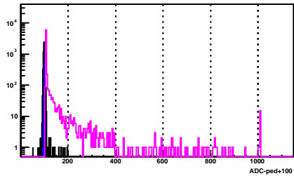
BSMD Strip 700_p
