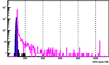
BSMD Strip 787_e
