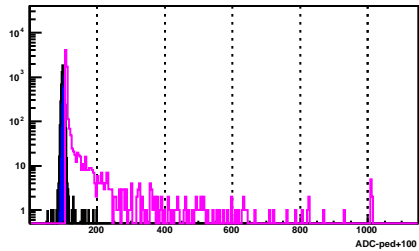
BSMD Strip 625_p
