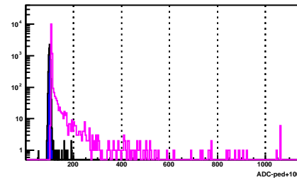
BSMD Strip 1374_e
