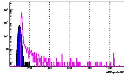
BSMD Strip 224_e
