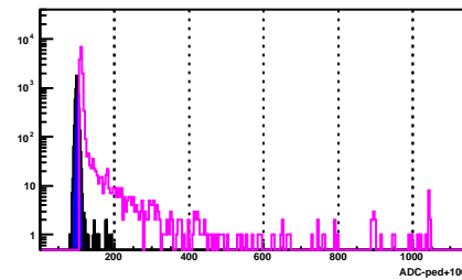
BSMD Strip 1860_e
