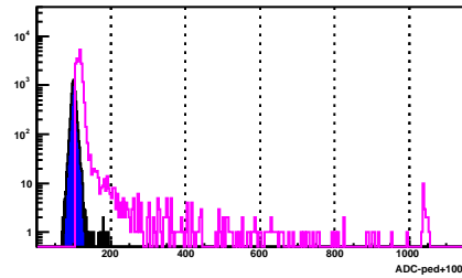
BSMD Strip 1910_e
