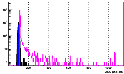
BSMD Strip 910_e
