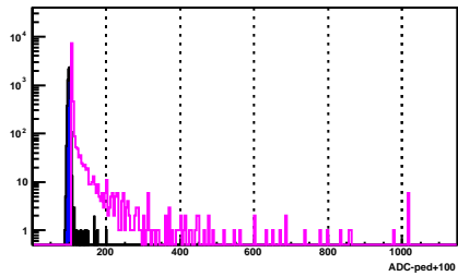
BSMD Strip 1210_e
