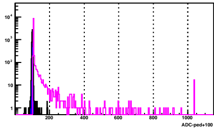
BSMD Strip 508_p
