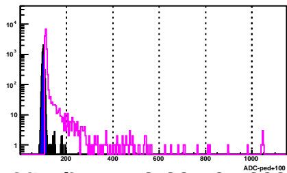
BSMD Strip 1858_e
