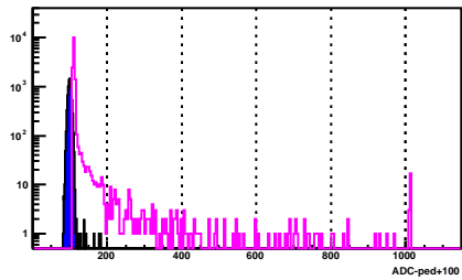
BSMD Strip 1297_e
