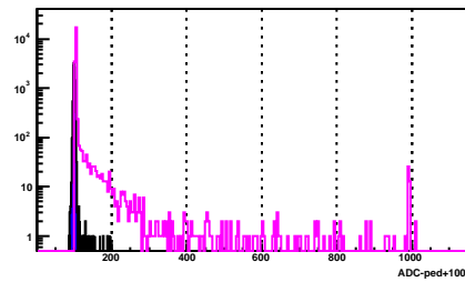
BSMD Strip 1334_e
