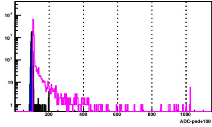
BSMD Strip 1663_e
