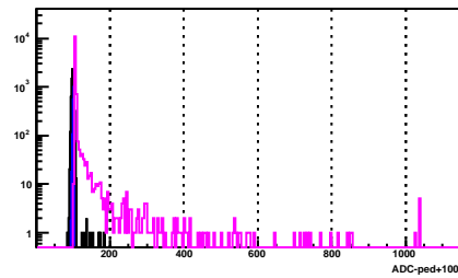
BSMD Strip 644_e
