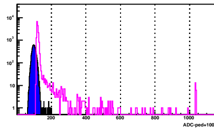
BSMD Strip 230_e
