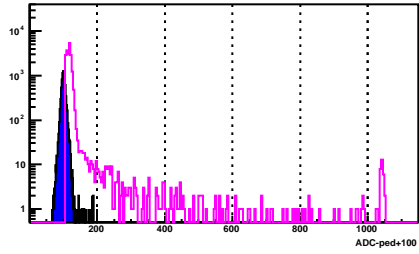
BSMD Strip 1912_e
