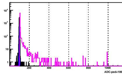
BSMD Strip 1619_p
