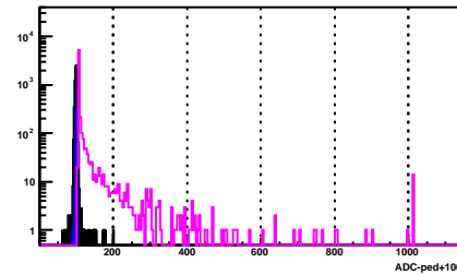
BSMD Strip 675_p
