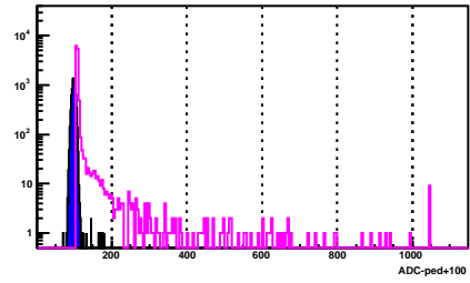
BSMD Strip 773_e
