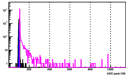
BSMD Strip 1765_p
