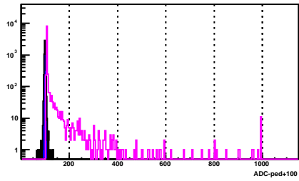
BSMD Strip 2080_p
