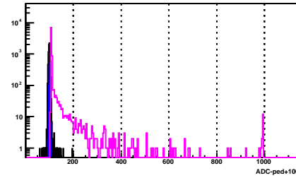
BSMD Strip 750_p
