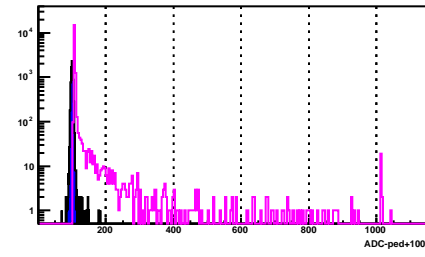
BSMD Strip 291_e
