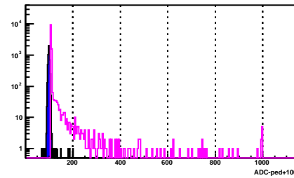
BSMD Strip 1674_p
