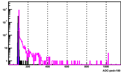
BSMD Strip 1060_e
