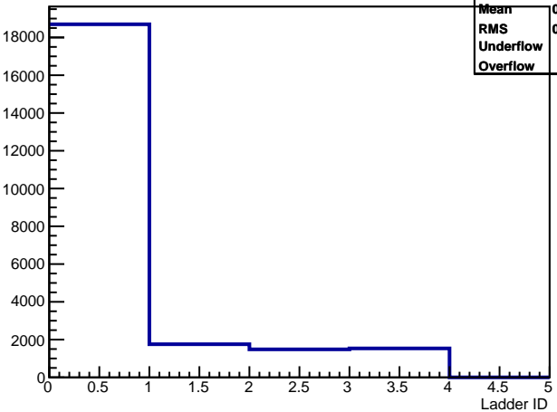
StE PIXEL: hits per ladder (per event)
