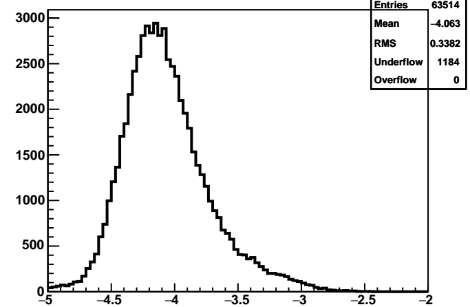
StE SST: log10(energy) of hits
