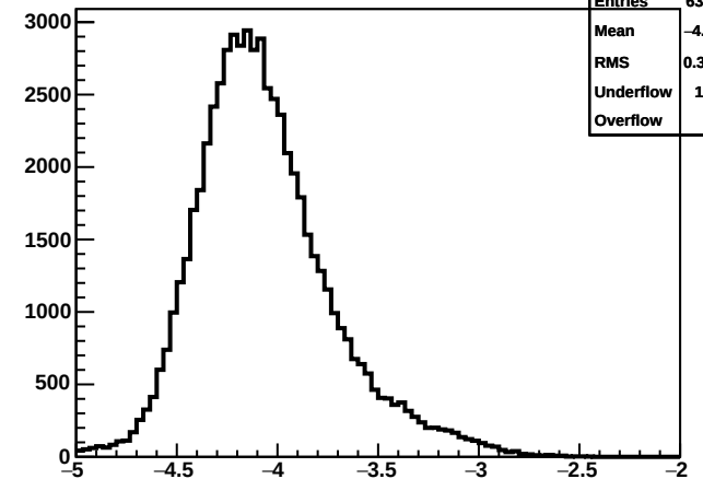
StE SST: \log_{10}(\text{energy}) of hits
