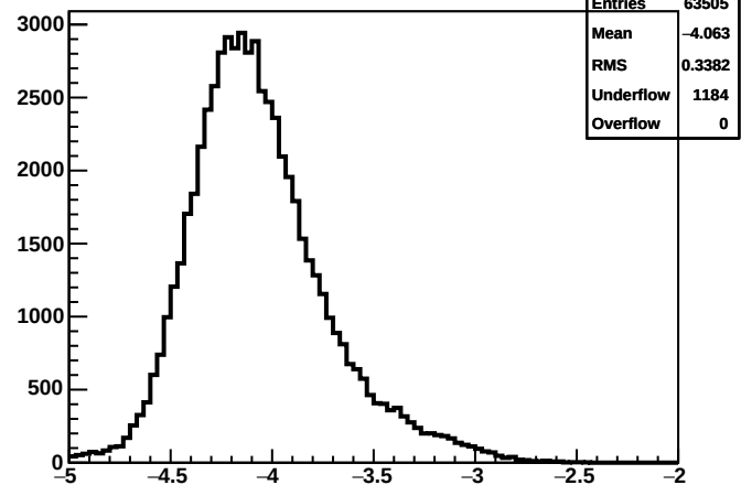
StE SST: log10(energy) of hits
