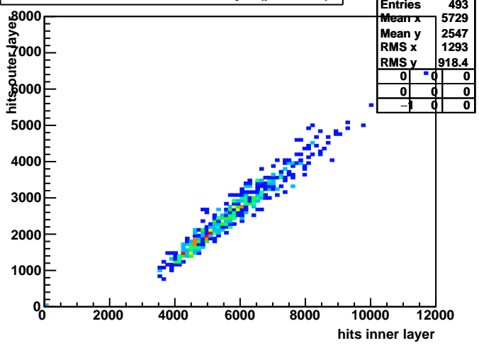
StE PIXEL: Hits in inner vs outer layer (per event)
