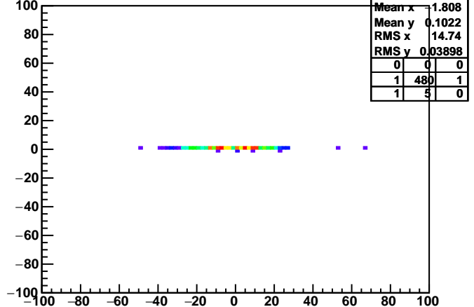
StE VPD vtx vs TPC vtx
