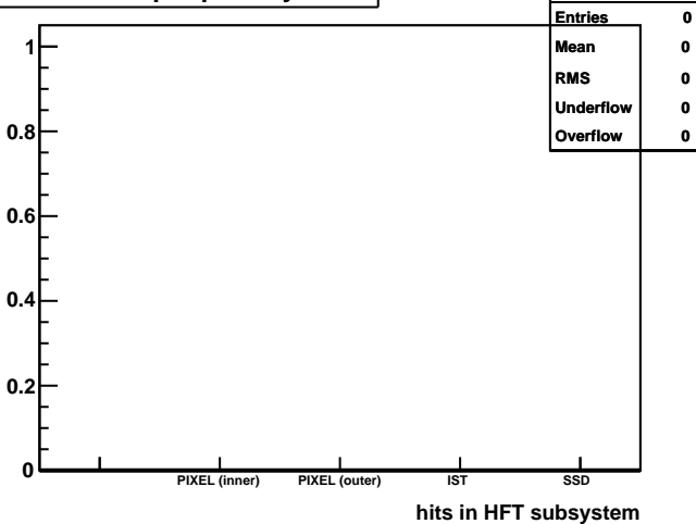
StE HFT: Hits per primary track
