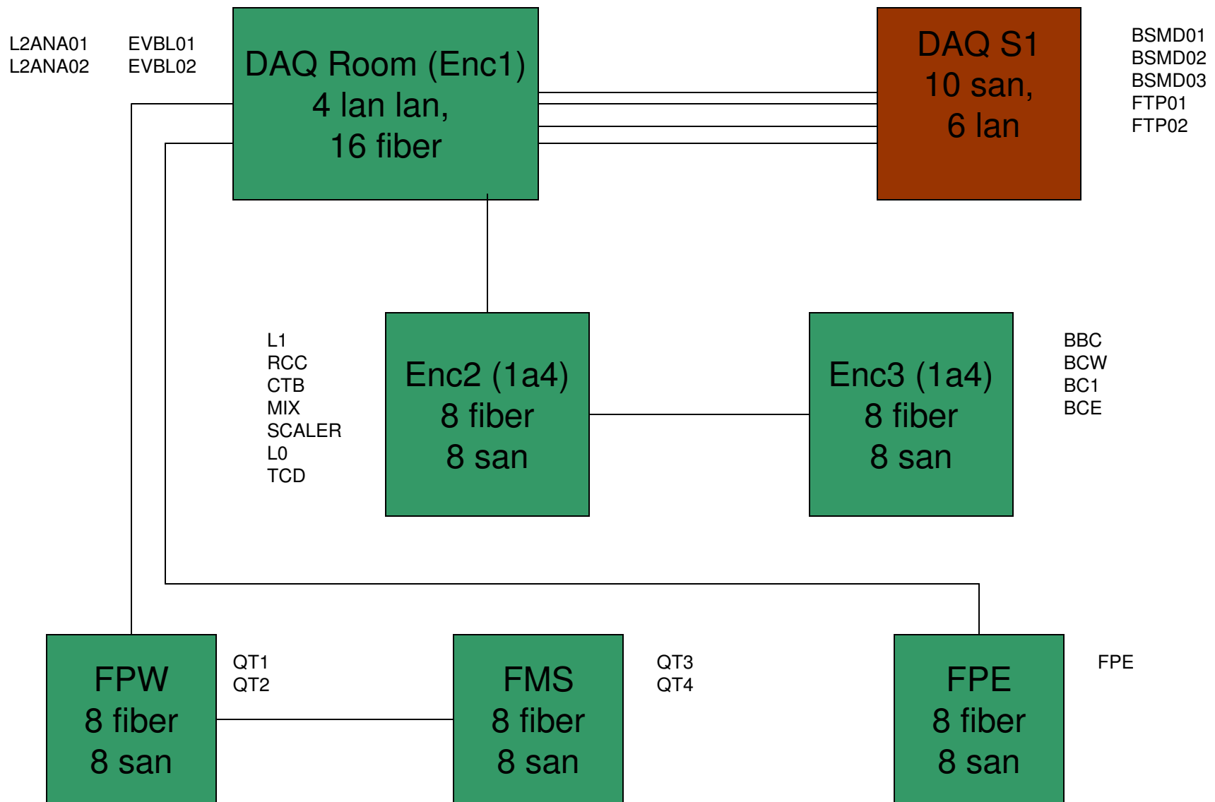
Proposed 2009 Myrinet Topology...
