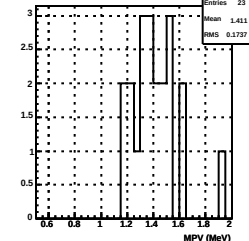
50 Mean of Landau fit to average MP ene (2019)
