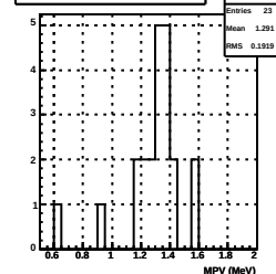
2V Mean of Landau fit to average MIP ene (2016)
