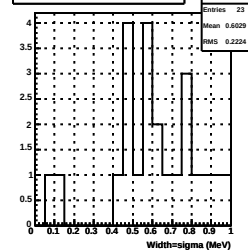
11V Width of Landau fit to average MIP ene (2016)
