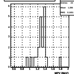
11U Mean of Landau fit to average MIP ene (2019)
