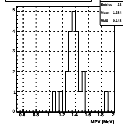
11V Mean of Landau fit to average MIP ene (2016)
