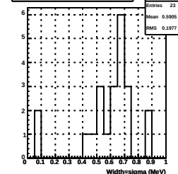
SDU Width of Landau fit to average MIP ene (2016)
