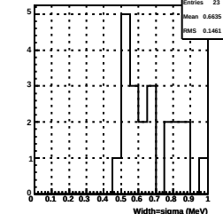
50 Width of Landau fit to average MP ene (2019)
