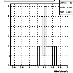
50% Mean of Landau fit to average MIP ene (2016)
