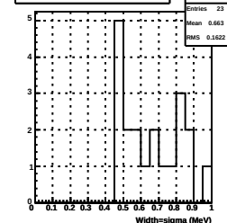
2V Width of Landau fit to average MIP ene (2016)
