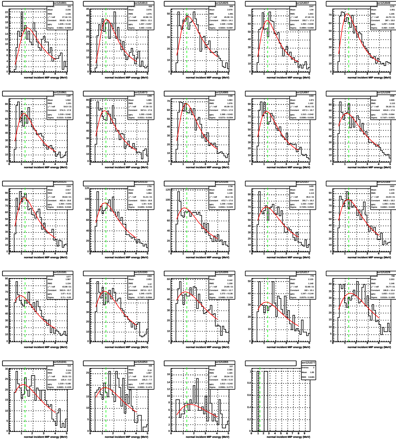
2U Mean of Landau fit to average MIP ene (2019)
