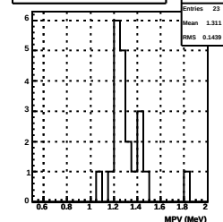
Plot Mean of Landau fit to average MIP ene (2016)
