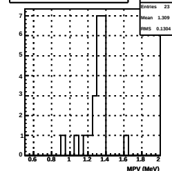
101 Mean of Landau fit to average MIP ene (2016)
