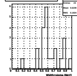
Plot Width of Landau fit to average MIP ene (2016)
