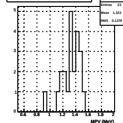
Mean of Landau fit to average MIP ene (2019)
