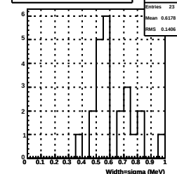
50% Width of Landau fit to average MIP ene (2019)
