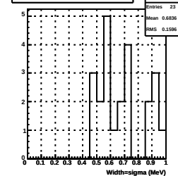
2U Width of Landau fit to average MIP ene (2019)
