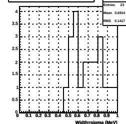
50% Width of Landau fit to average MIP ene (2016)
