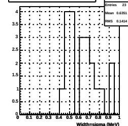
101 Width of Landau fit to average MIP ene (2016)
