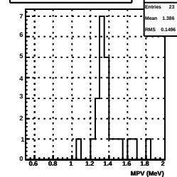
2U Mean of Landau fit to average MIP ene (2019)
