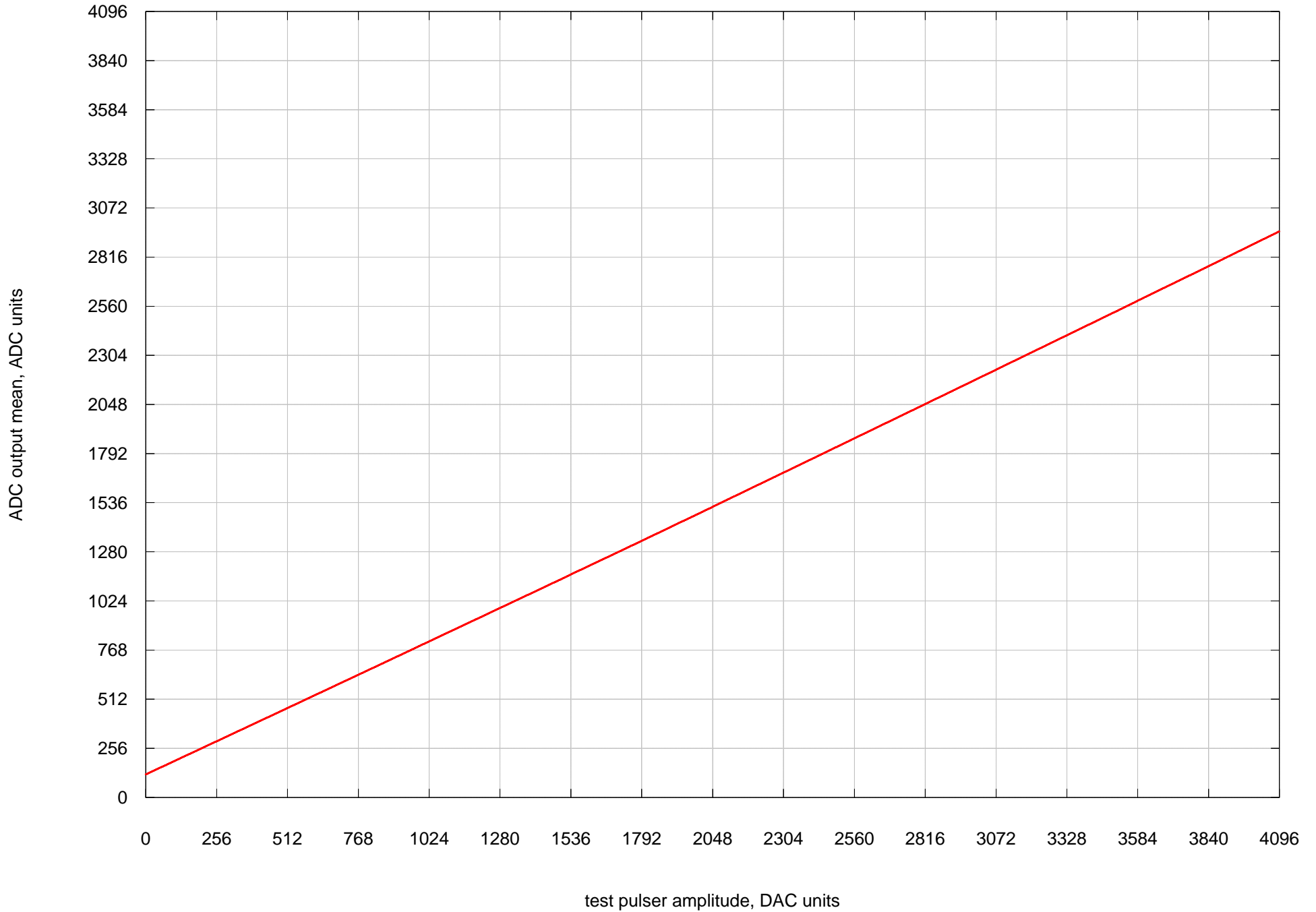
chan 90 internal test pulser response vs. amplitude
