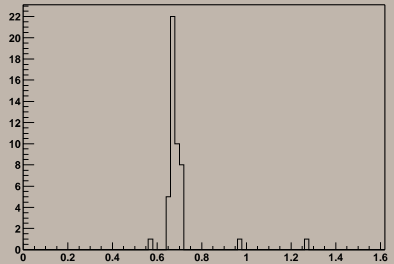
Sigma (fit) in ADC response, all channels
