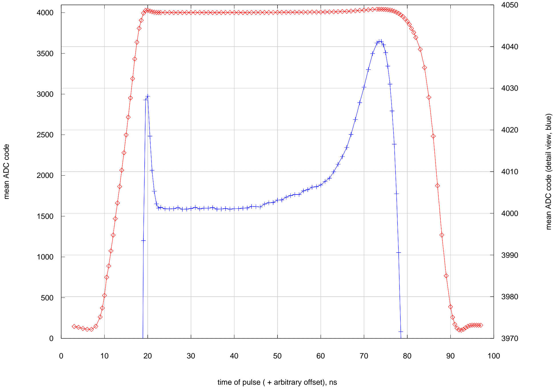
FEE prototype pulser response vs. time of pulse
