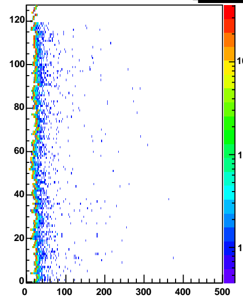
cr2 Entries 101632
