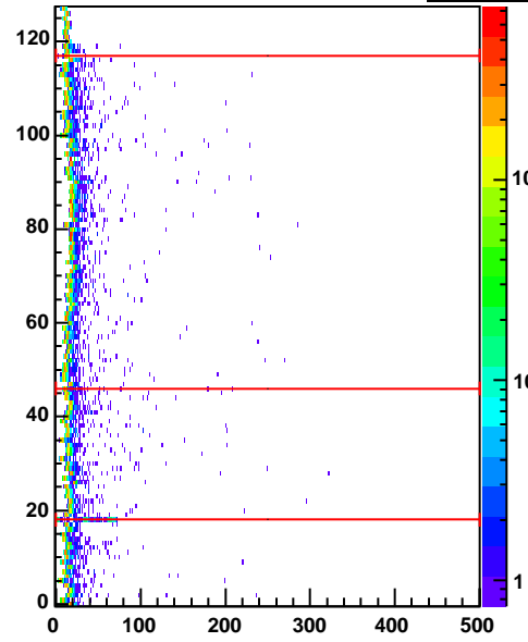
cr4 Entries 101632
