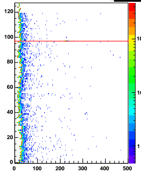
cr1 Entries 101632
