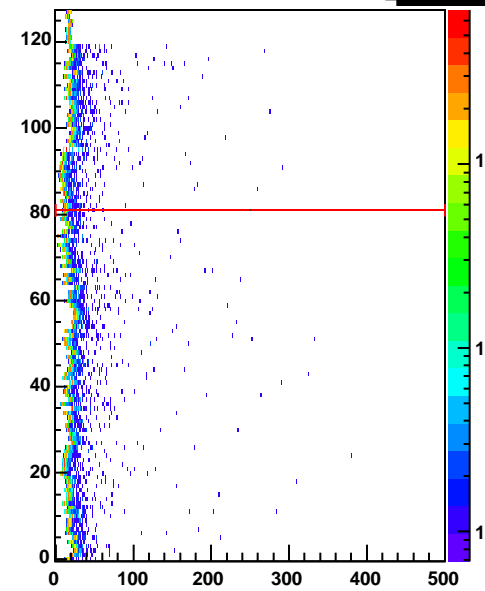
cr3 Entries 101632
