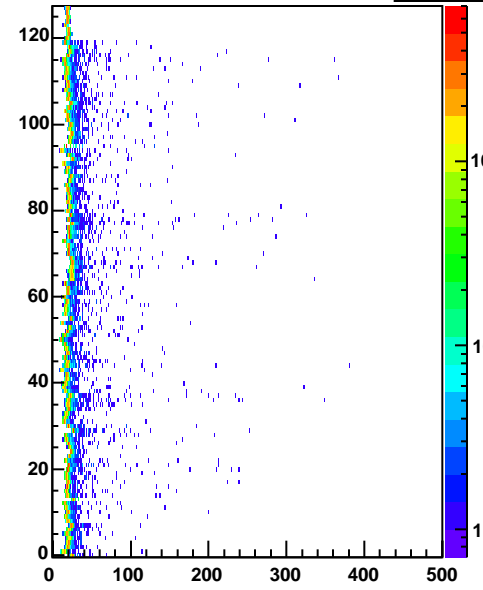
cr5 Entries 101632
