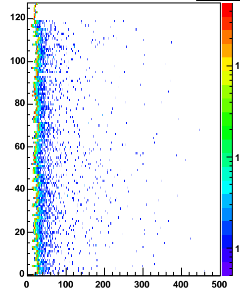
cr6 Entries 101632
