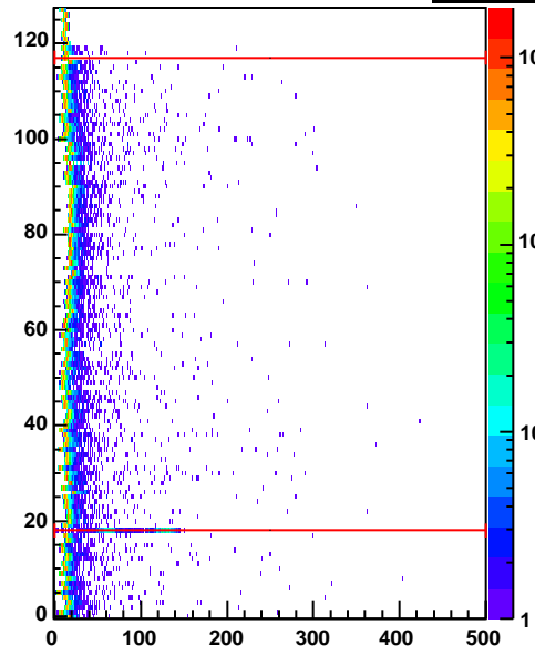
cr4 Entries 265728
