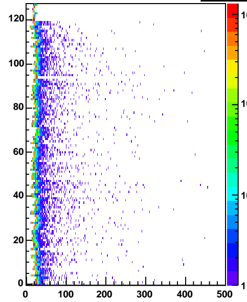
cr6 Entries 265728
