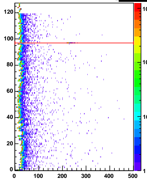
cr1 Entries 265728
