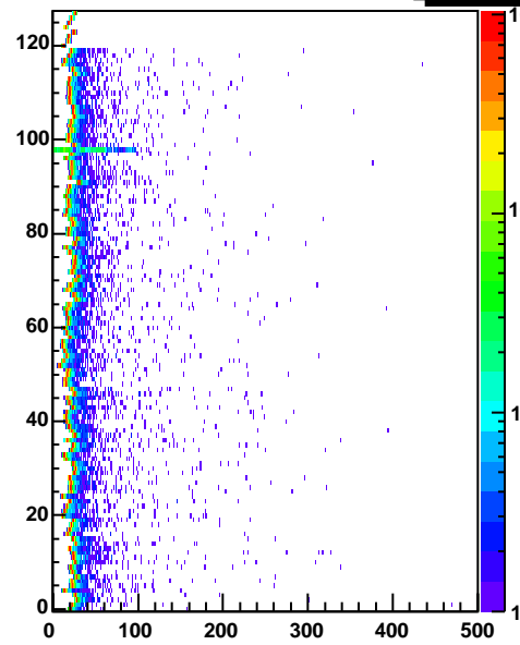
cr2 Entries 265728
