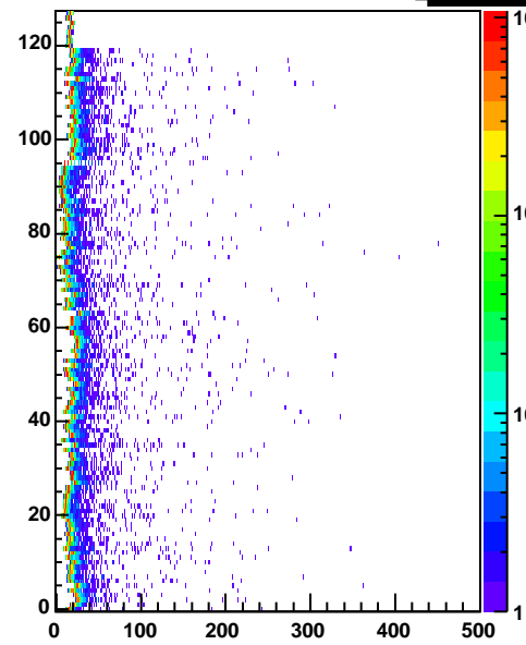
cr3 Entries 265728
