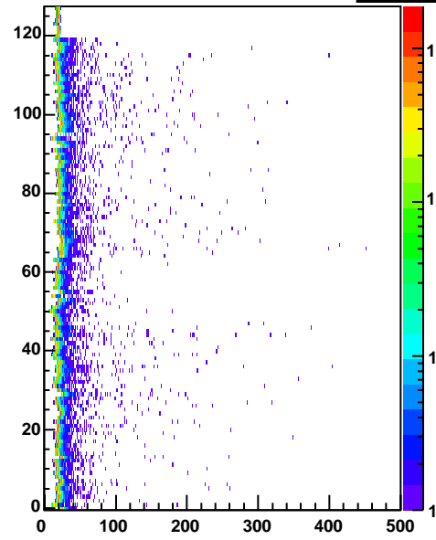
cr5 Entries 265728
