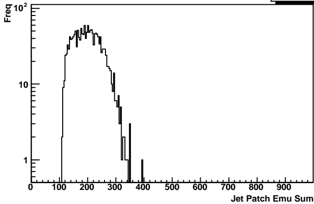
Emulated Sum Jet Patches 5+6
