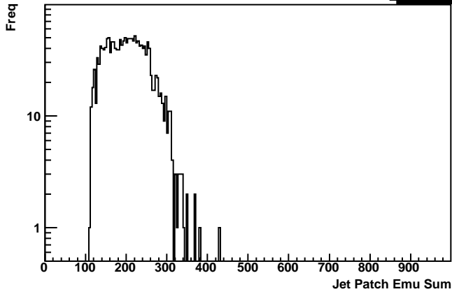
Emulated Sum Jet Patches 3+4
