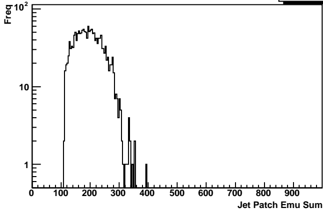
Emulated Sum Jet Patches 5+6
