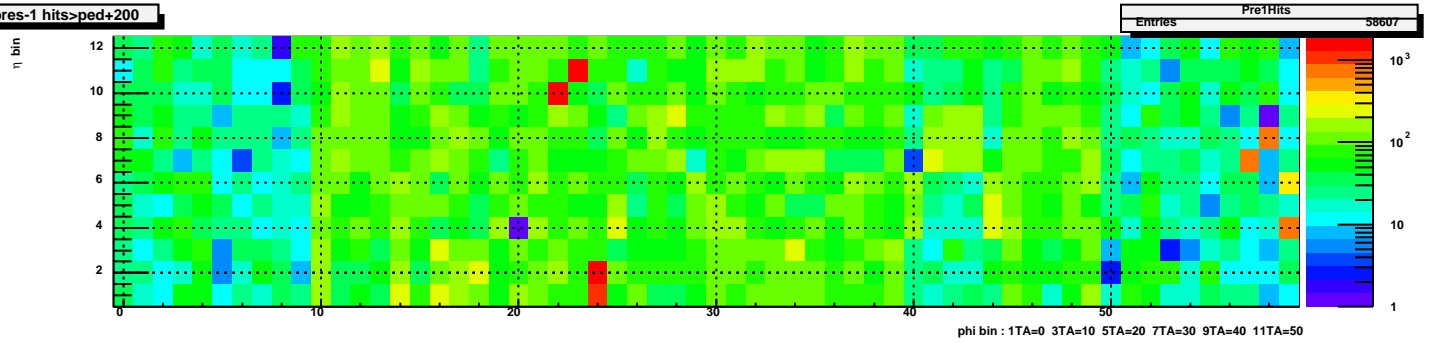
pres-2 hits>ped+200
