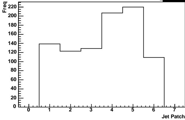
Emu Jet Patch over software Thr1=62
