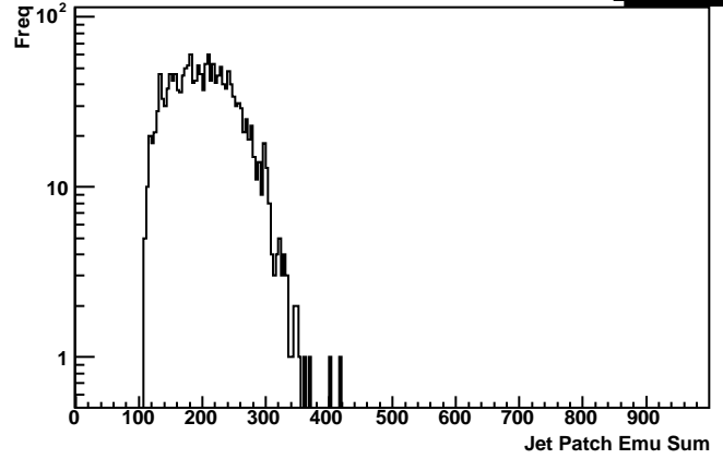
Emulated Sum Jet Patches 4+5
