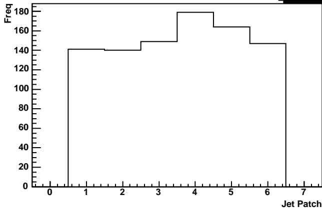
Adjacent Jet patches both over thr0
