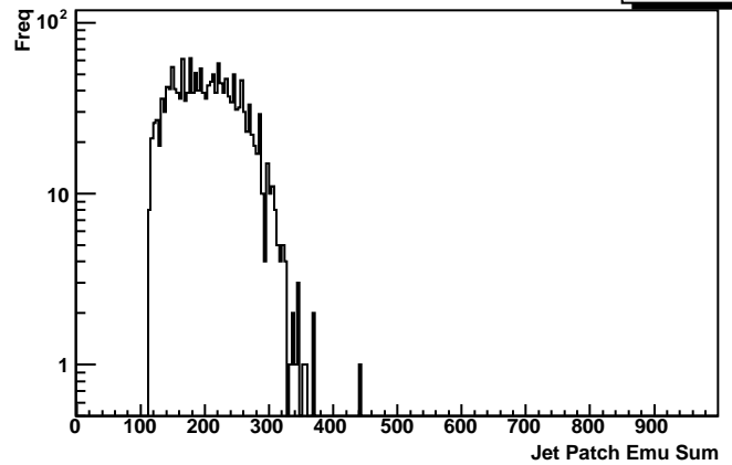
Emulated Sum Jet Patches 6+1
