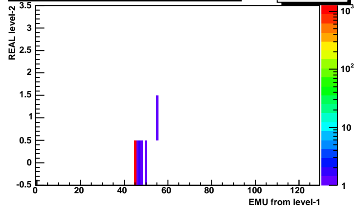
TP inp vs. emu, layer-2, JP_Falk(3), trig=allTrig
