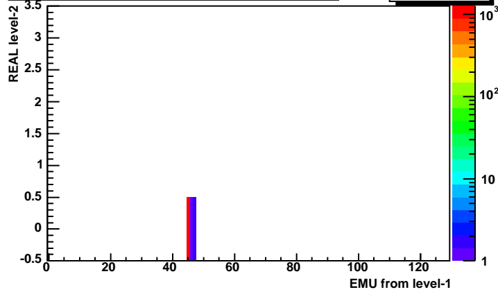
TP inp vs. emu, layer-2, JP_Falk(0), trig=allTrig
