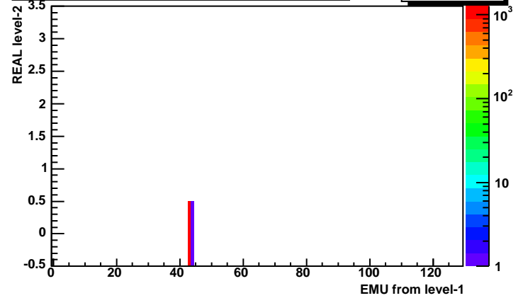
TP inp vs. emu, layer-2, JP_Falk(1), trig=allTrig
