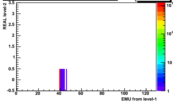
TP inp vs. emu, layer-2, JP_Falk(2), trig=allTrig
