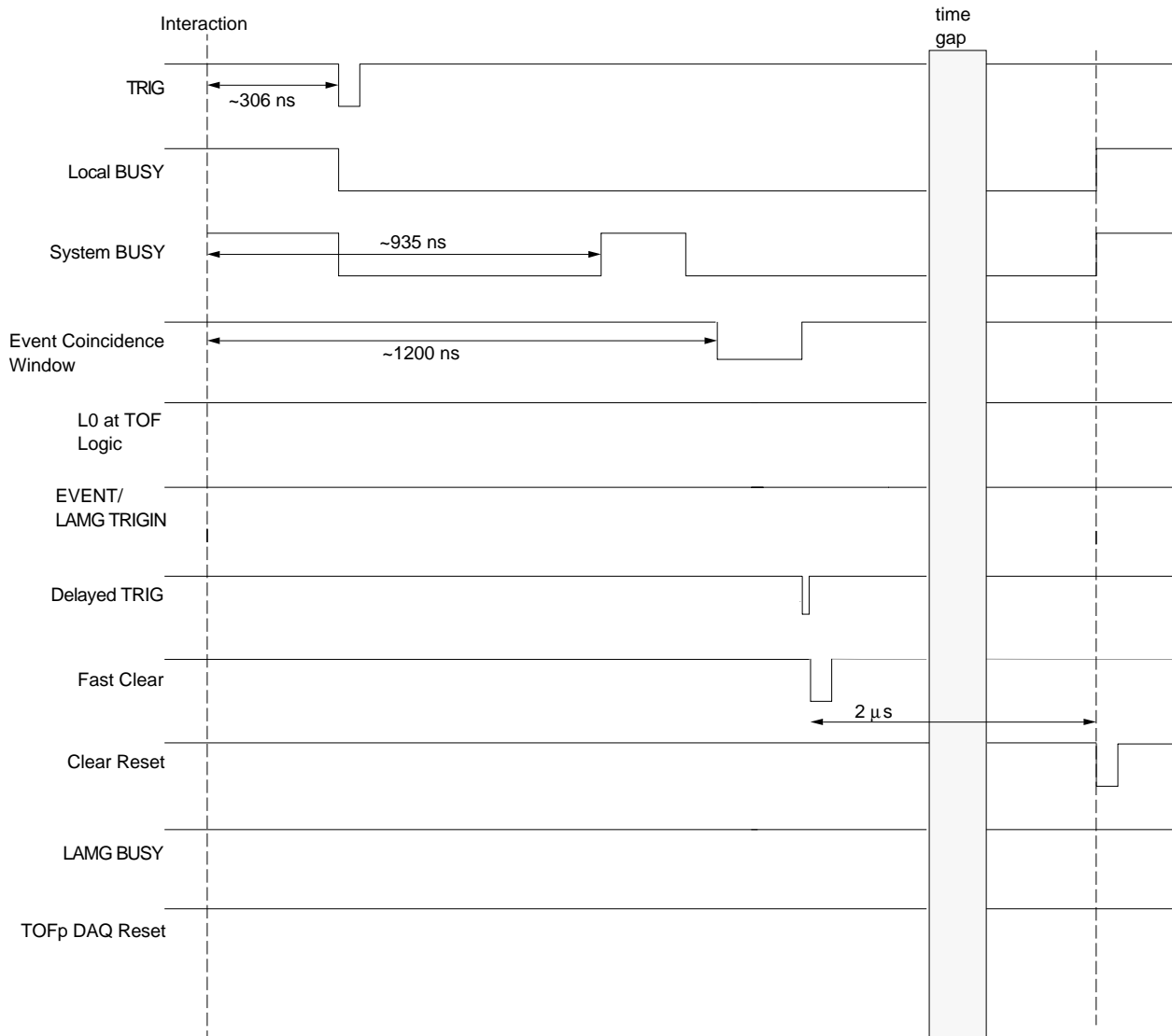
Bad Event (no L0) Timing Diagram Pulser enabled running with 25 April 2001 Logic
