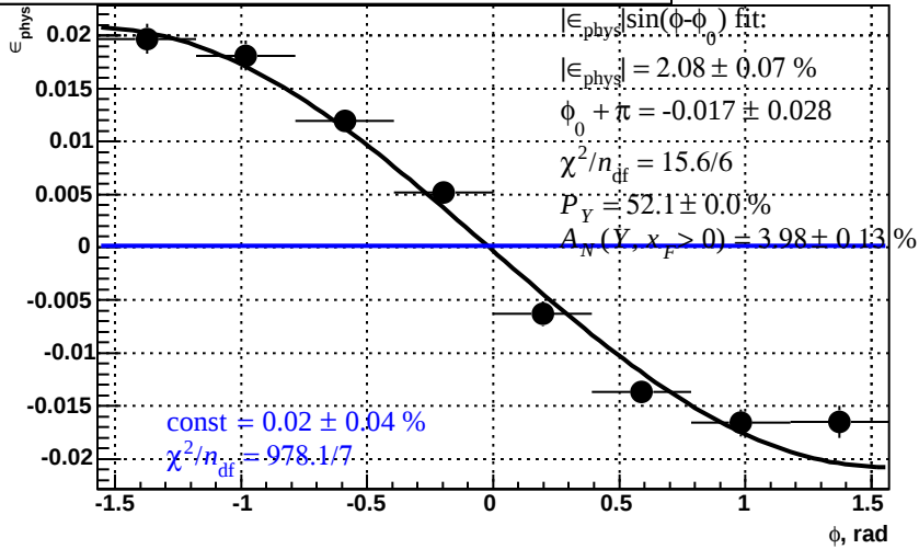
Square root asymmetry vs. \phi , Blue Forward (West)
