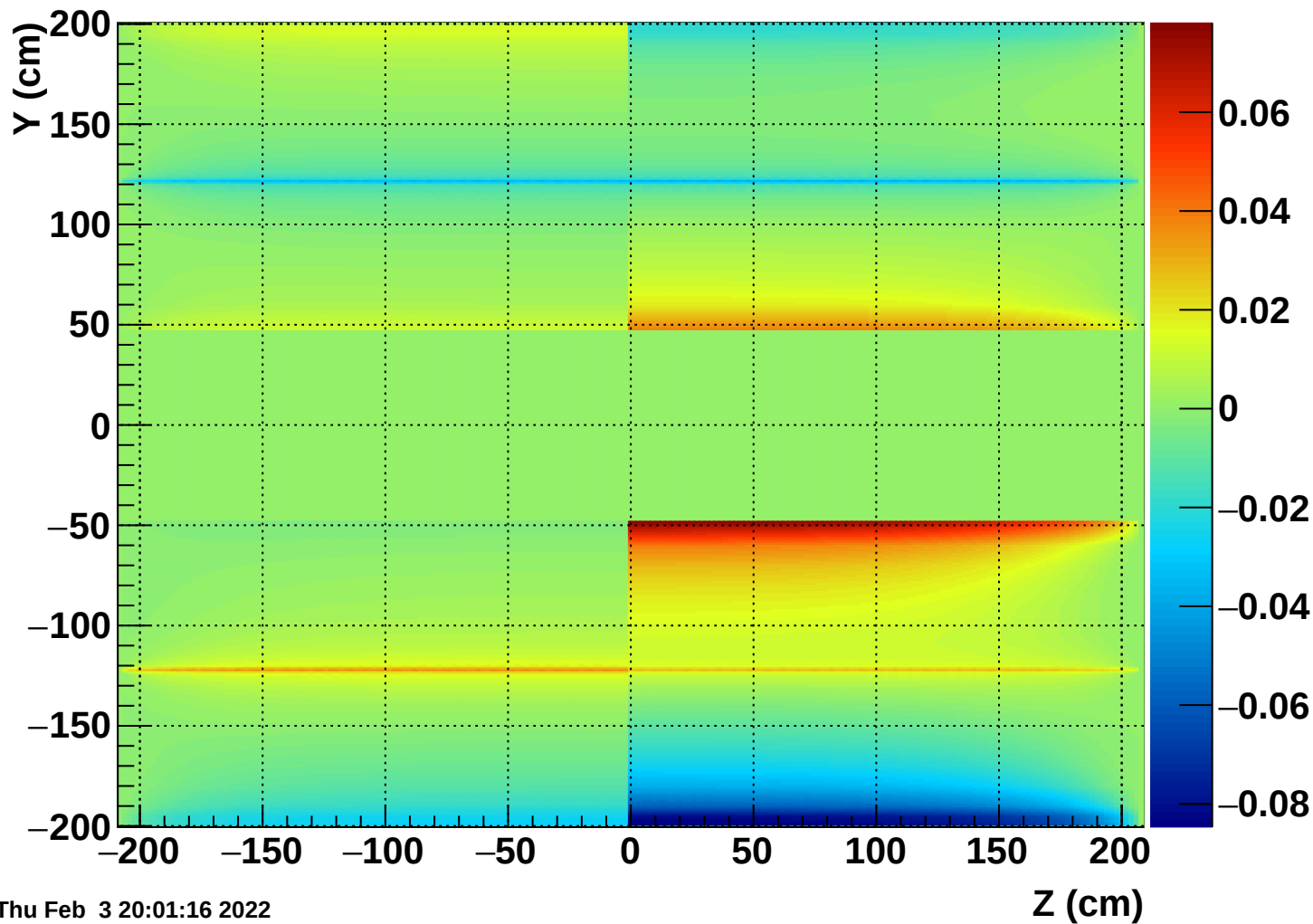
dX (cm) at X = 0 for OSectorAlign and AuAu200_2019
