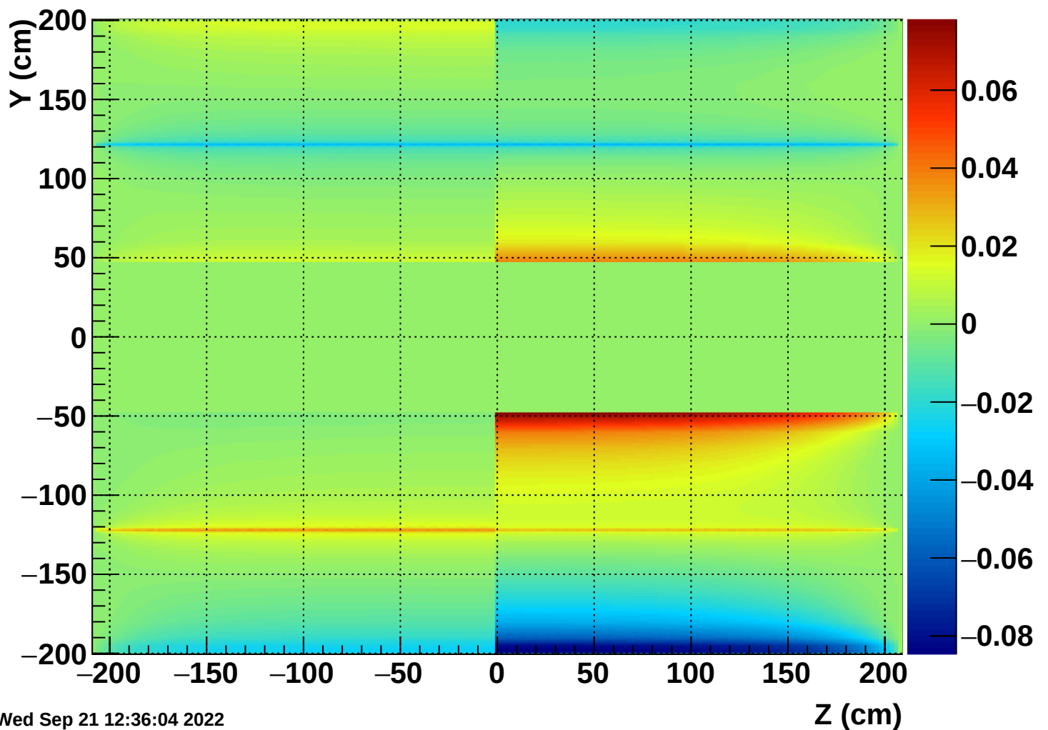
dX (cm) at X = 0 for OSectorAlign and 7p7GeV_2021DbV
