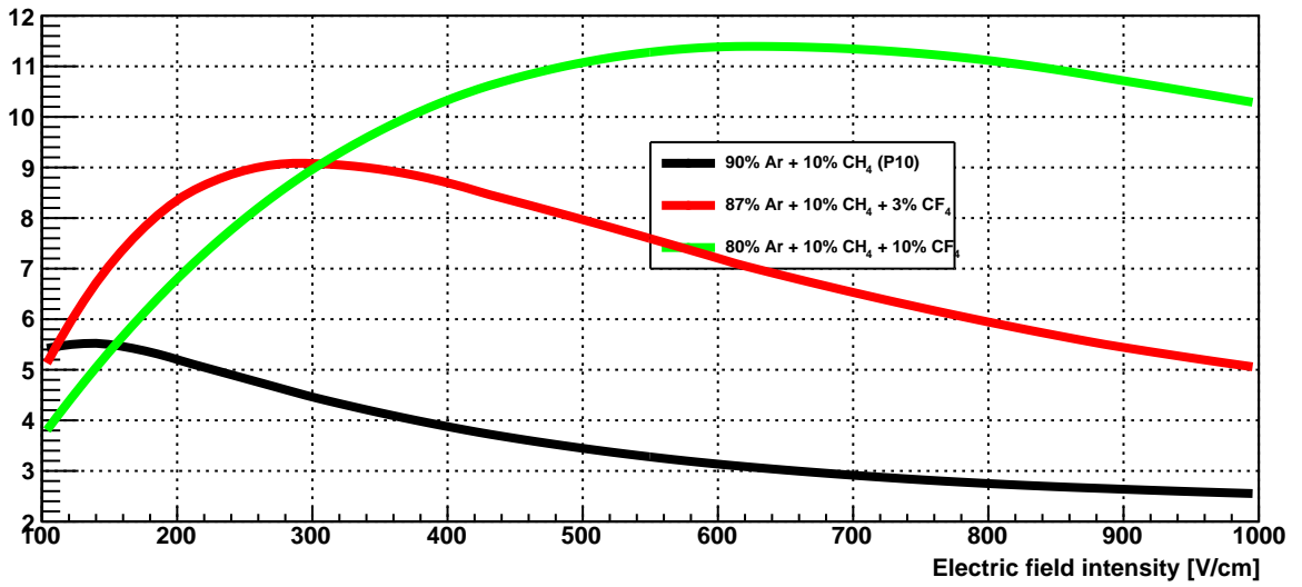
Electron drift velocity [cm/ \mu sec] versus electric field intensity
