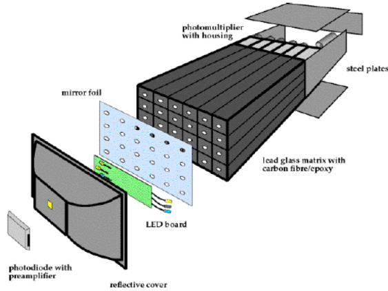
Figure 3.20.: A PbG1 supermodule showing the arrangement of towers and PMTs.
