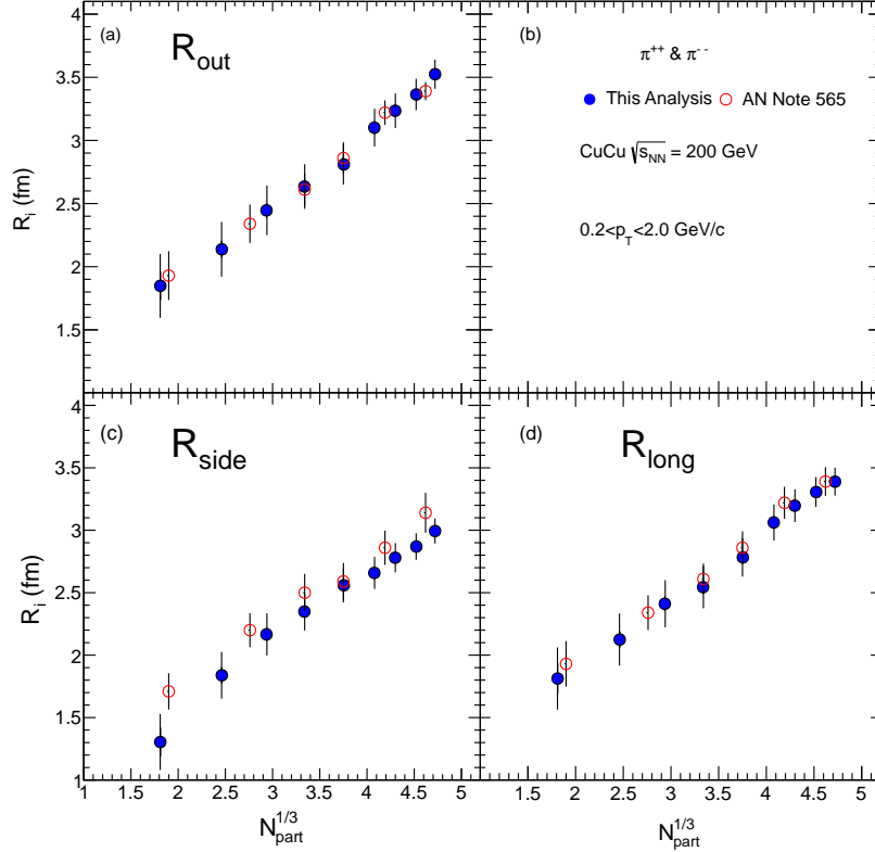
Figure 5.3.: Comparison of these results with previous PHENIX results for Cu + Cu at \sqrt{s_{NN}} = 200 GeV.
