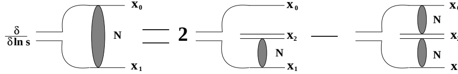
Figure 5.10. Diagrammatic representation of the nonlinear evolution equation (5.13).
