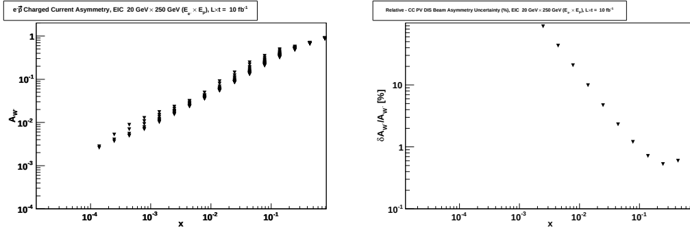
Figure 1.37. Left: spin asymmetry for CC e^- \bar{p} scattering, as function of x for various bins in Q^2 . Right: resulting relative uncertainties of the asymmetry.
