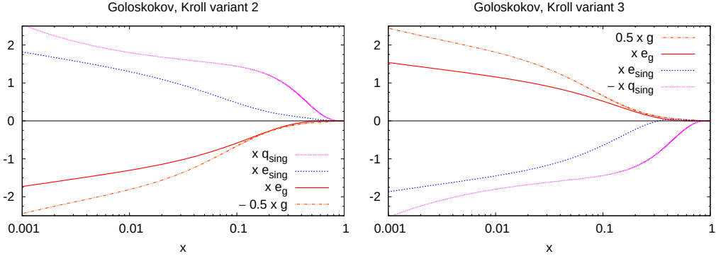
Figure 3.13. Two variants of model distributions e_g and e_{\text{sing}} at \mu = 2 \text{ GeV} from [605]. The distributions of the quark singlet q_{\text{sing}} = \sum_q (q + \bar{q}) and the gluon are shown for comparison.
