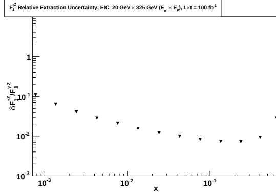
Figure 1.43. Same as left part of Fig. 1.42, but for \vec{e}^-D scattering.
