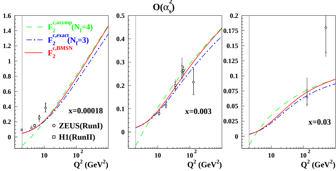
Figure 1.14. Comparison of F_2^c computed in different schemes to H1 and ZEUS data: GMVFNS in the BMSN prescription (solid lines), 3-flavor scheme (dot-dashed lines), and 4-flavor scheme (dashed lines). The vertical dotted line denotes the position of m_c = 1.43 GeV. Taken from Ref. [19].
