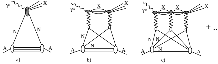
Figure 5.34. The multiple scattering series for the \gamma^* A \rightarrow X A diffractive scattering amplitude. Graph a is the impulse approximation; graphs b and c correspond to the interaction with two and three nucleons of the nuclear target, and contribute to the shadowing correction.
