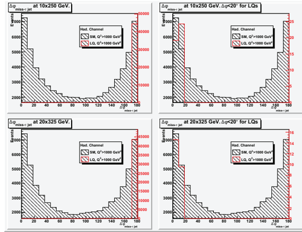
Figure 6.18. Acoplanarity \Delta\phi_{miss,\tau_{jet}} at 10 \times 250 and 20 \times 325 GeV with Q^2 > 1000 \text{ GeV}^2 . The two plots in the right side have a \Delta\phi < 20^\circ cut implemented on the LQ simulation. In this case, the LQ preserves the quark flavor: ( q_i = 1 \ q_j = 1 ). These plots are not normalized amongst themselves.
