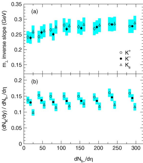
Fig. 2. The centrality dependence of (a) kaon inverse slopes and (b) mid-rapidity kaon to negative hadron ratios. The error bars are uncorrelated random errors; correlated systematic errors are indicated by the shaded areas. An additional systematic error (not shown) of 5% and 7% applies to the dN/dy of kaons and dN_{h^-}/d\eta , respectively. For clarity the K^+ and K_S^0 points are displaced in dN_{h^-}/d\eta .
