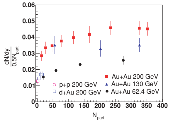
FIG. 12. (Color online) N_{\text{part}} dependence of (dN/dy)/0.5N_{\text{part}} in five different collision systems: Au + Au 62.4, 130, 200 GeV; p + p 200 GeV (inelastic); and d + \text{Au} 200 GeV. Statistical and systematic errors are included.
