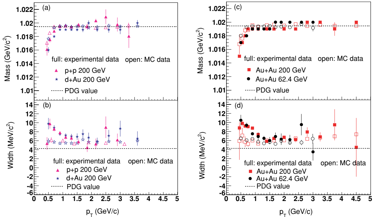
FIG. 8. (Color online) Masses and widths (FWHMs) of \phi as a function of p_T in p + p 200 GeV (NSD), d + \text{Au} 200 GeV (0–20%), Au + Au 62.4 GeV (0–20%), and Au + Au 200 GeV (0–5%) collisions, with the corresponding PDG values.
