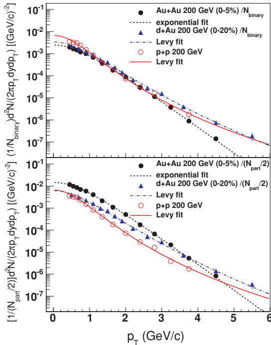
FIG. 11. (Color online) Comparison of transverse momentum spectra shape among different 200 GeV collision systems: Au + Au (0–5%), d + \text{Au} (0–20%), and p + p (inelastic). The spectra are normalized by N_{\text{bin}} (top panel) and N_{\text{part}}/2 (bottom panel).
