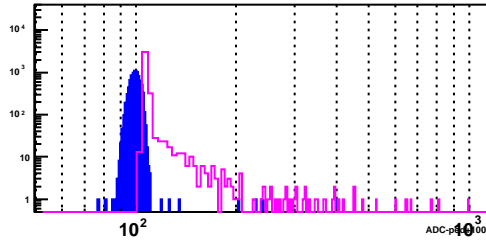
BSMD Strip 2921_p
