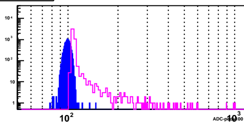
BSMD Strip 2909_p
