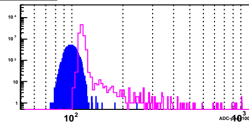
BSMD Strip 2982_e
