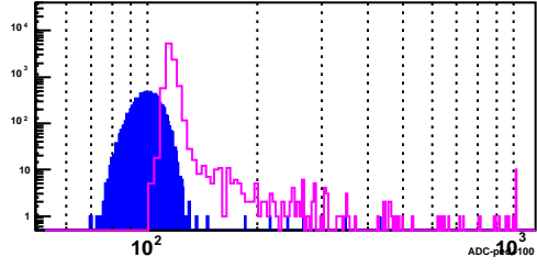
BSMD Strip 2992_e
