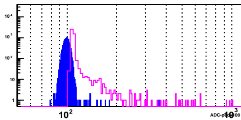
BSMD Strip 2900_p
