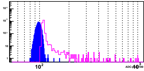
BSMD Strip 2863_p
