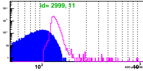
BSMD Strip 2999_e
