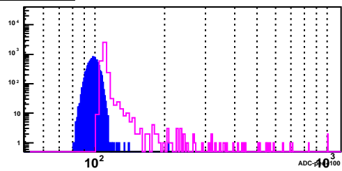
BSMD Strip 2878_p
