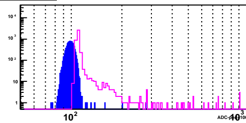
BSMD Strip 2880_p
