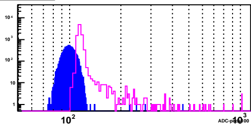
BSMD Strip 2984_e
