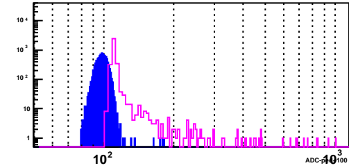
BSMD Strip 2865_p
