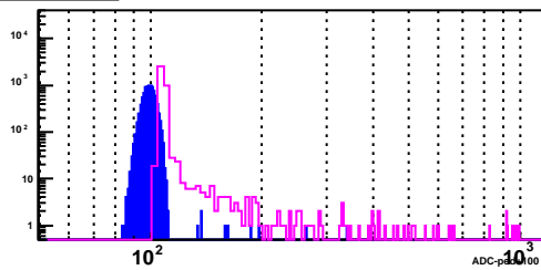
BSMD Strip 2903_p
