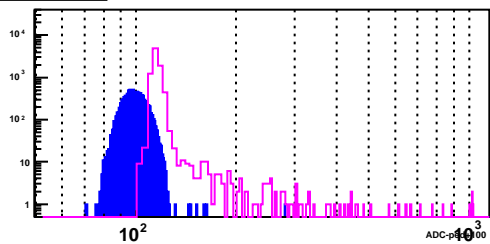
BSMD Strip 2981_e
