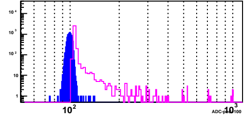
BSMD Strip 2919_p
