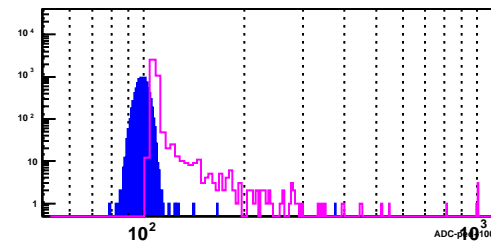
BSMD Strip 2901_p
