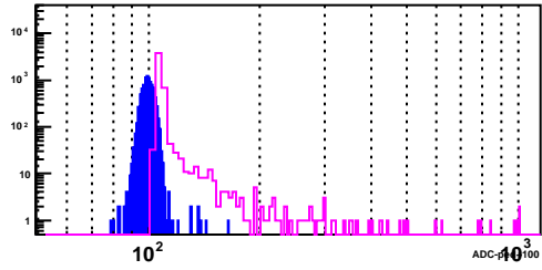
BSMD Strip 2920_p
