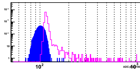
BSMD Strip 2916_e
