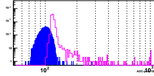
BSMD Strip 2994_e
