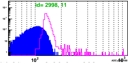
BSMD Strip 2998_e
