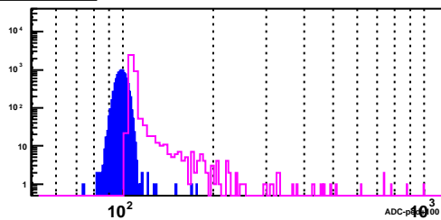
BSMD Strip 2906_p
