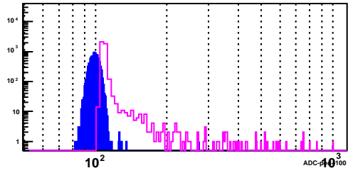
BSMD Strip 2914_p
