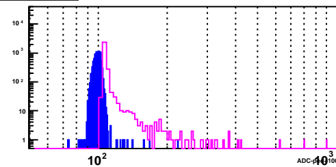
BSMD Strip 2907_p
