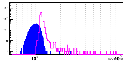
BSMD Strip 2925_e
