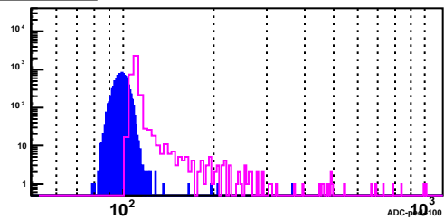
BSMD Strip 2872_p
