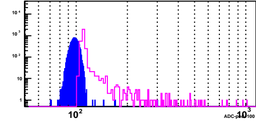
BSMD Strip 2859_p
