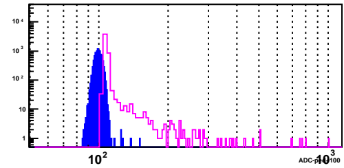
BSMD Strip 2925_p
