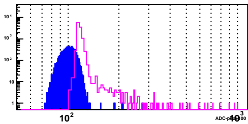
BSMD Strip 2915_e
