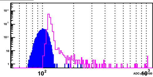
BSMD Strip 2920_e
