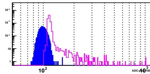
BSMD Strip 2976_e
