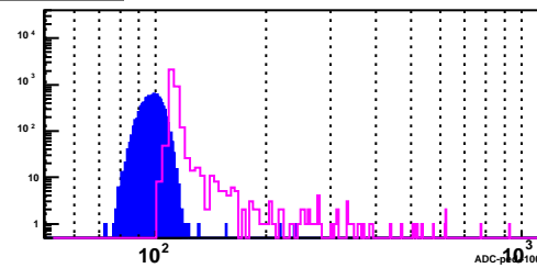
BSMD Strip 2874_p
