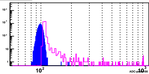
BSMD Strip 2873_p
