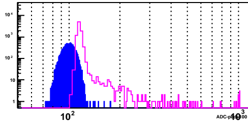
BSMD Strip 2990_e
