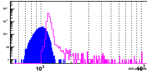
BSMD Strip 2996_e
