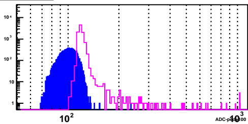
BSMD Strip 2924_e
