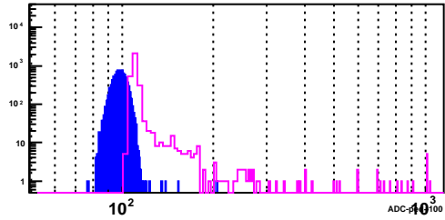
BSMD Strip 2860_p
