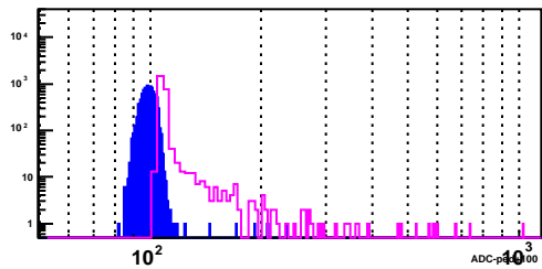
BSMD Strip 2894_p
