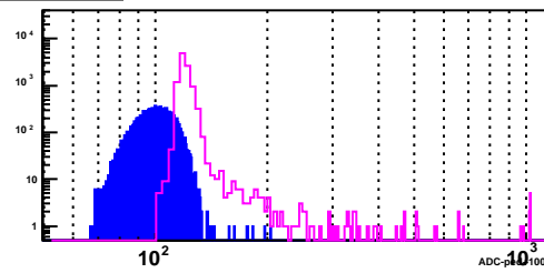
BSMD Strip 2934_e
