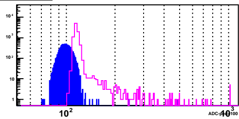
BSMD Strip 2983_e
