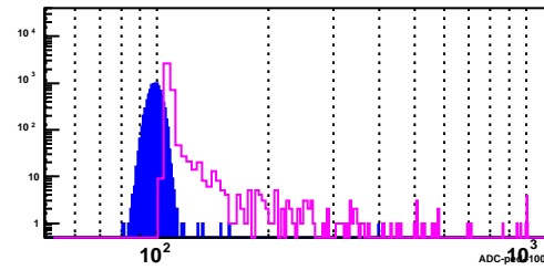
BSMD Strip 2889_p
