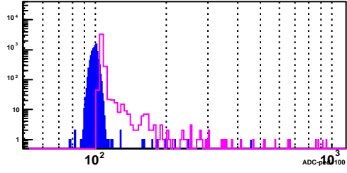
BSMD Strip 2917_p
