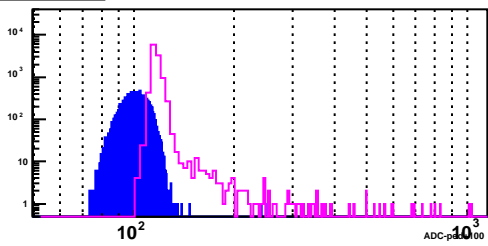
BSMD Strip 2918_e
