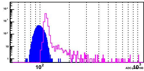
BSMD Strip 2977_e
