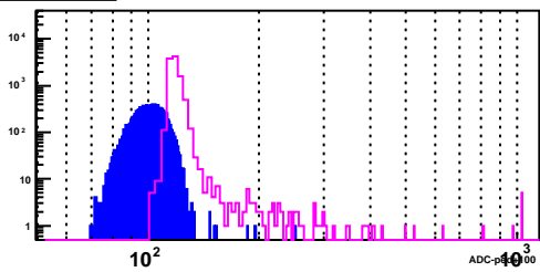
BSMD Strip 2921_e
