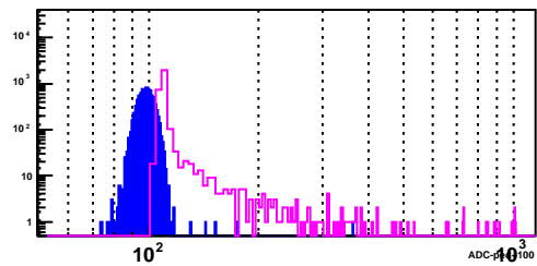
BSMD Strip 2869_p
