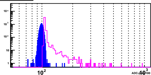
BSMD Strip 2908_p
