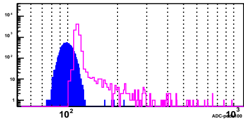
BSMD Strip 2978_e
