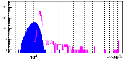
BSMD Strip 2995_e
