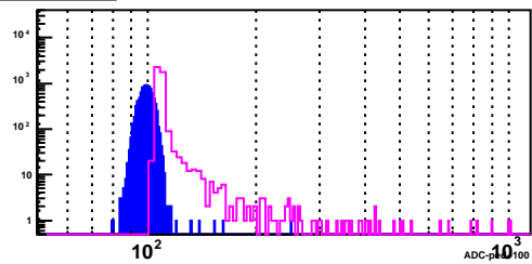
BSMD Strip 2902_p
