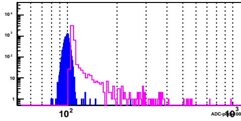
BSMD Strip 2915_p
