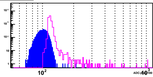
BSMD Strip 2923_e
