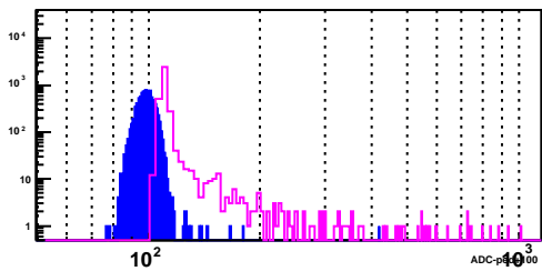
BSMD Strip 2870_p
