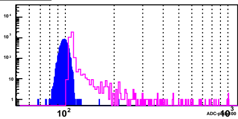
BSMD Strip 2879_p
