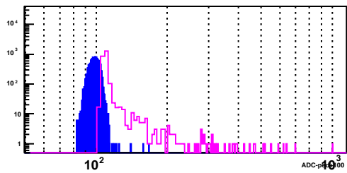
BSMD Strip 2885_p
