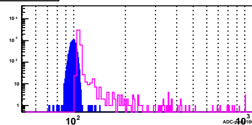
BSMD Strip 2910_p
