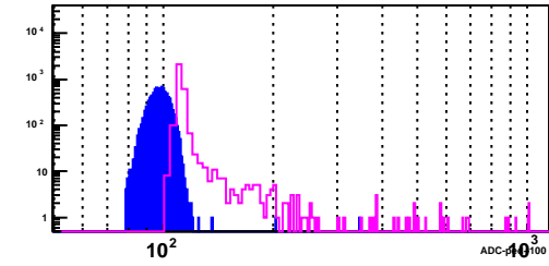
BSMD Strip 2856_p
