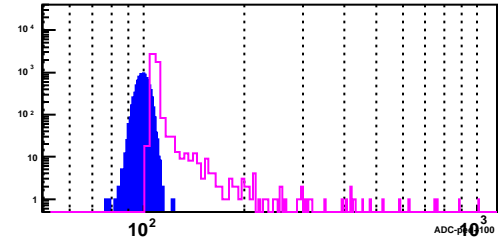
BSMD Strip 2922_p
