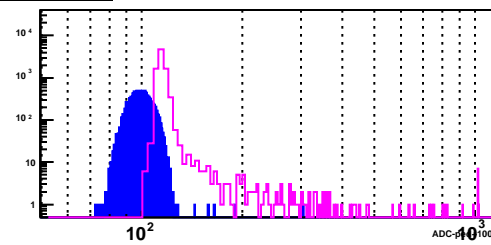
BSMD Strip 2985_e
