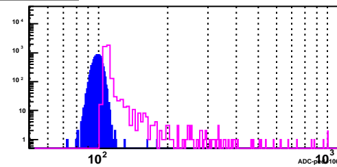
BSMD Strip 2904_p
