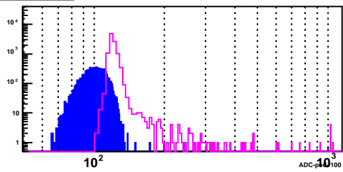
BSMD Strip 2932_e
