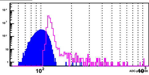
BSMD Strip 2939_e
