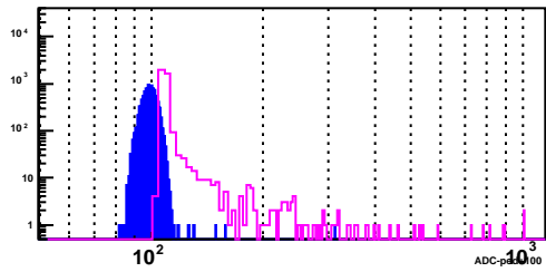
BSMD Strip 2888_p
