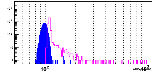
BSMD Strip 2862_p
