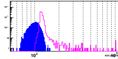
BSMD Strip 2997_e
