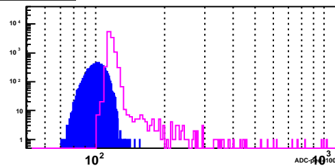
BSMD Strip 2922_e
