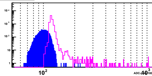
BSMD Strip 2940_e
