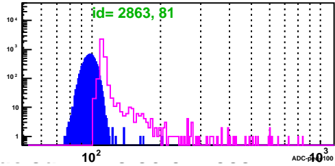
BSMD Strip 2863_p
