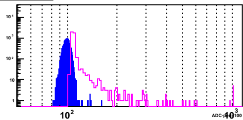
BSMD Strip 2890_p
