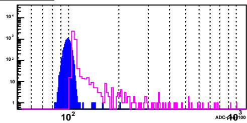
BSMD Strip 2893_p
