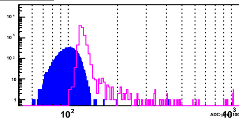
BSMD Strip 2937_e
