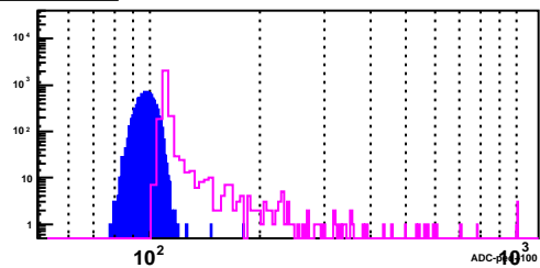
BSMD Strip 2875_p
