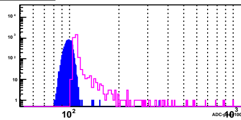
BSMD Strip 2895_p
