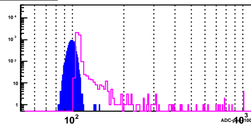
BSMD Strip 2892_p
