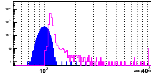
BSMD Strip 2991_e
