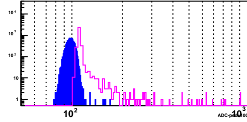
BSMD Strip 2858_p
