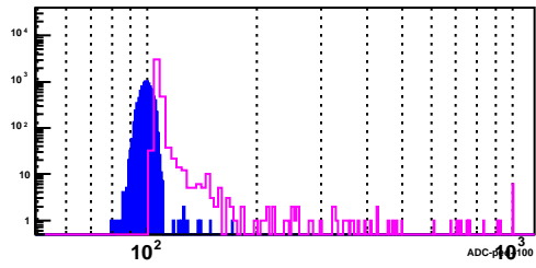
BSMD Strip 2923_p
