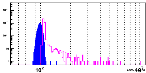
BSMD Strip 2891_p
