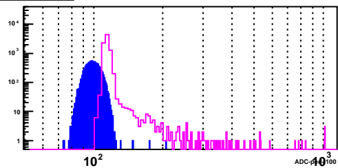
BSMD Strip 2980_e
