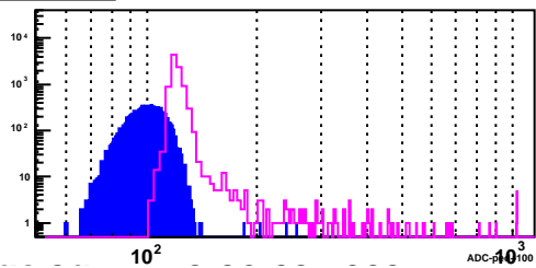
BSMD Strip 2938_e
