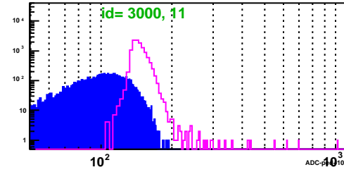
BSMD Strip 3000_e
