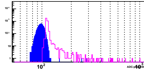
BSMD Strip 2864_p
