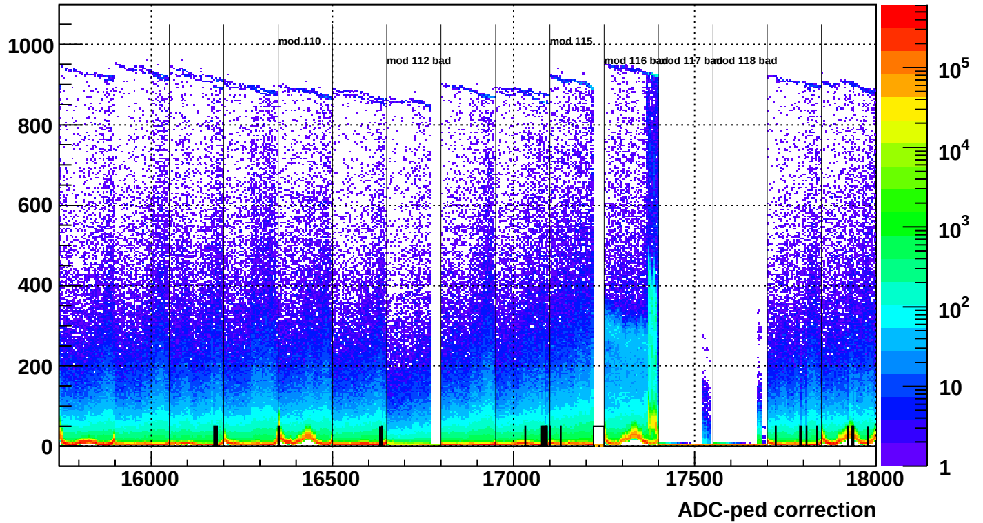
bsmdep ZS ADC-onIPed for modules 106 to 120
