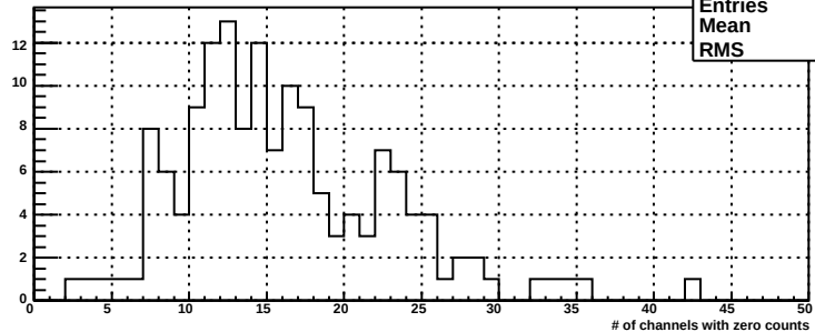
nlow for bsm dp plane, mod 114
