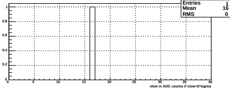
nlow for bsmde plane, mod 114
