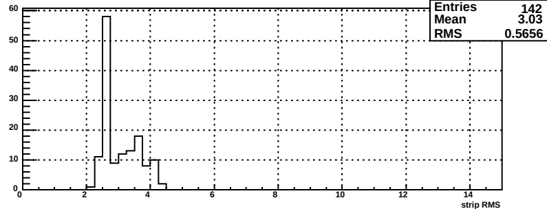
rms for bsmde plane, mod 114
