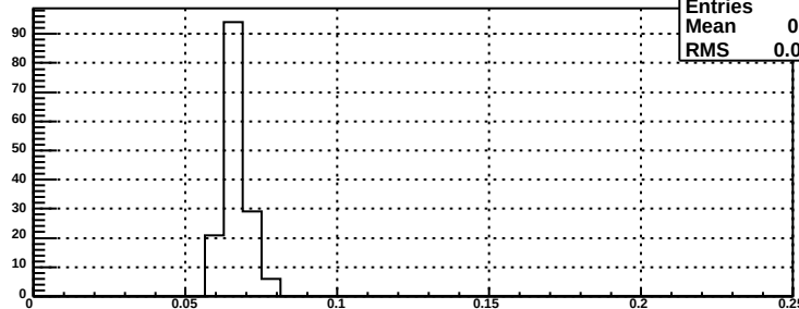
relative errors for bsm dp plane, mod 114
