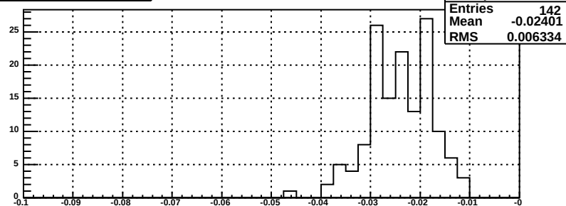
slopes for bsmde plane, mod 114
