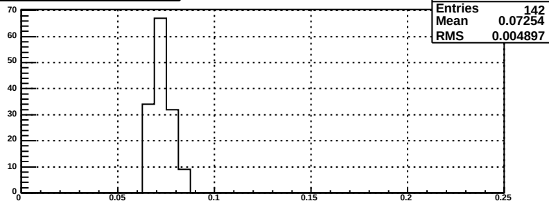
relative errors for bsmde plane, mod114
