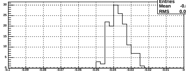
slopes for bsm dp plane, mod 114
