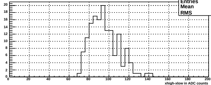
rms for bsm dp plane, mod 114
