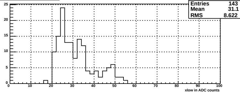
xlow for bsmde plane, mod 119
