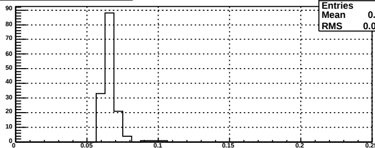
relative errors for bsm dp plane, mod 119
