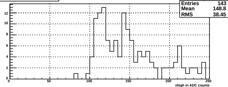
xhigh for bsmde plane, mod 119
