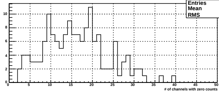
nzero for bsm dp plane, mod 119
