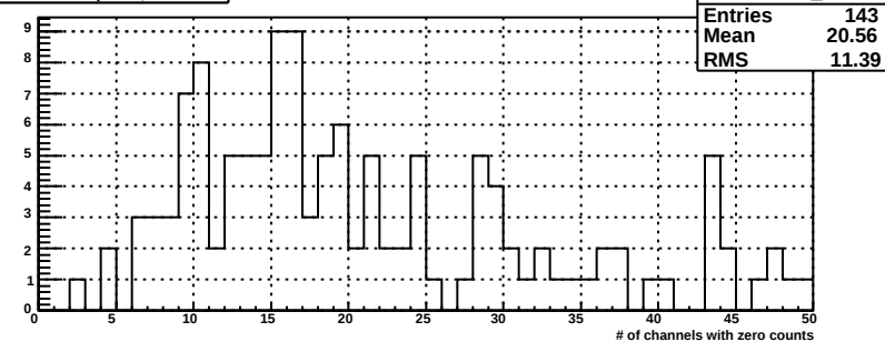
nzero for bsmde plane, mod 119
