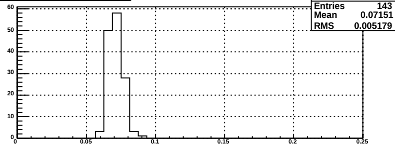
relative errors for bsmde plane, mod119
