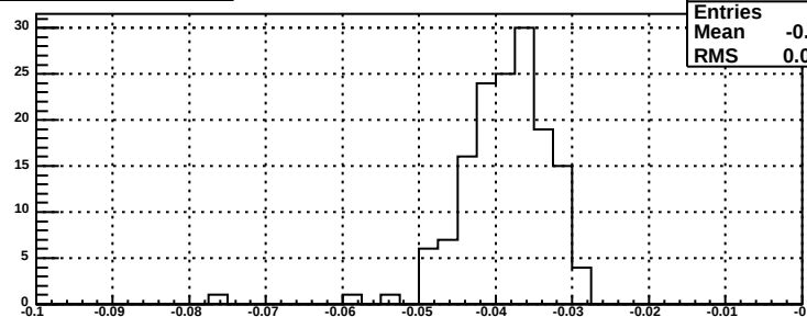
slopes for bsm dp plane, mod 119
