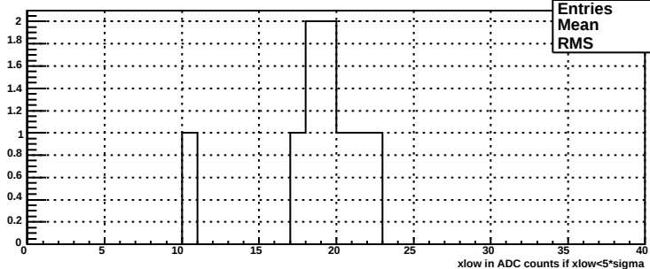
nlow for bsm dp plane, mod 119
