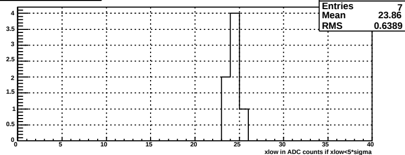
nlow for bsmde plane, mod 119
