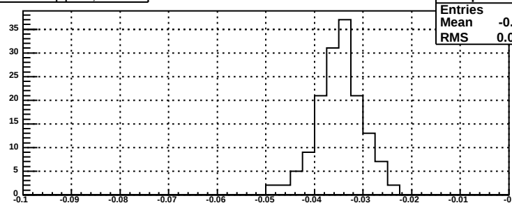
slopes for bsm dp plane, mod 120
