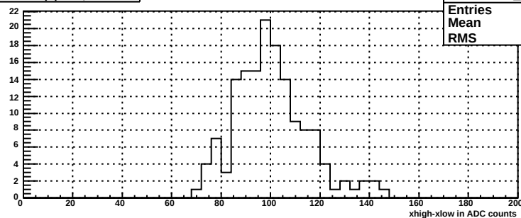
xdiff for bsm dp plane, mod 120
