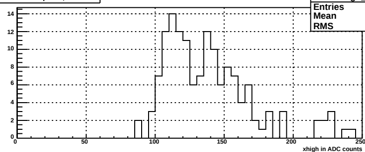
xhigh for bsmde plane, mod 111
