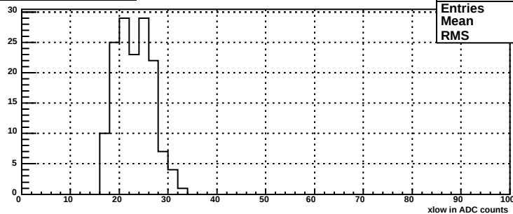
xlow for bsm dp plane, mod 111
