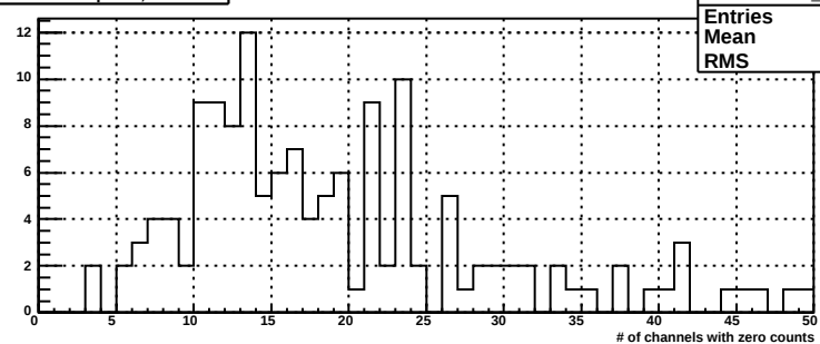
nzero for bsmde plane, mod 111
