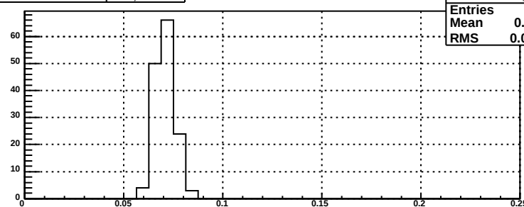
relative errors for bsmde plane, mod 111
