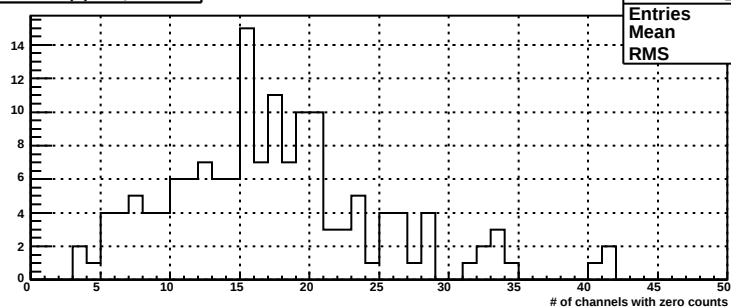
nzero for bsm dp plane, mod 111
