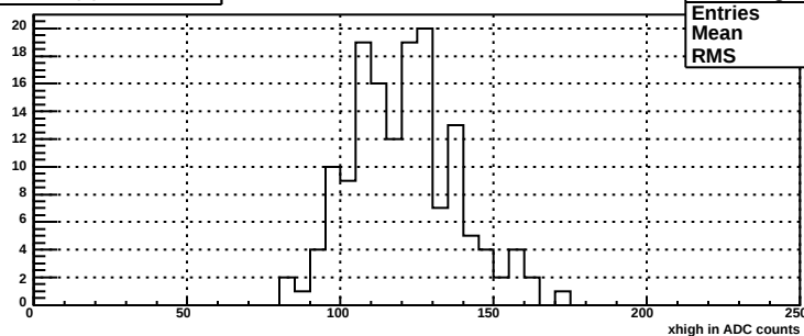
xhigh for bsm dp plane, mod 111
