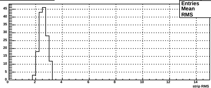
rms for bsm dp plane, mod 111
