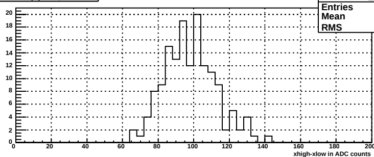
xdiff for bsm dp plane, mod 111
