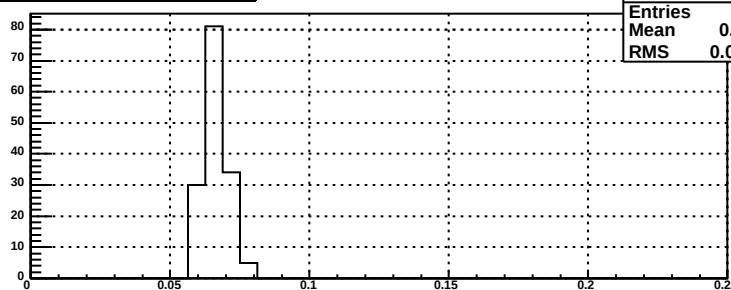
relative errors for bsm dp plane, mod 111
