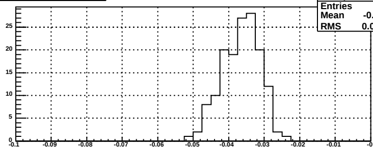
slopes for bsm dp plane, mod 111
