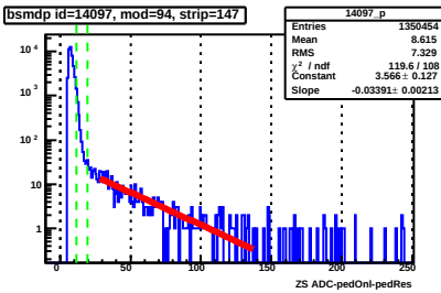
bsmdp id=14097, mod=94, strip=147
