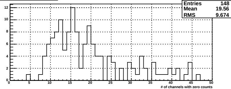
nzero for bsmde plane, mod 99
