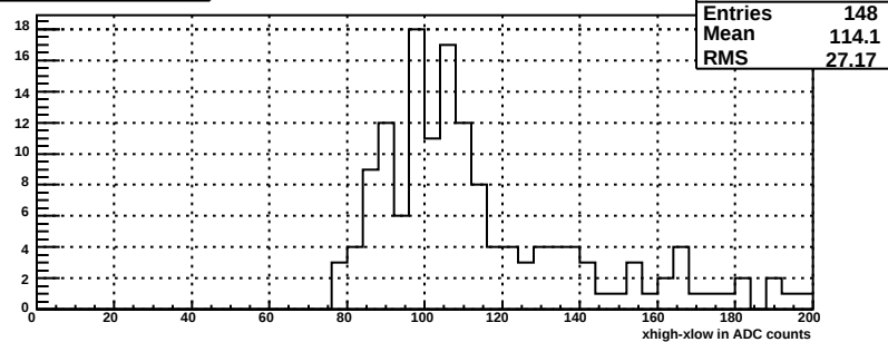
xdiff for bsmde plane, mod 99
