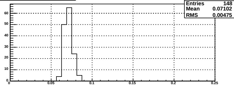
relative errors for bsmde plane, mod99
