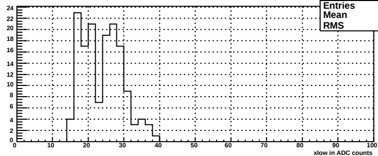
xlow for bsm dp plane, mod 99
