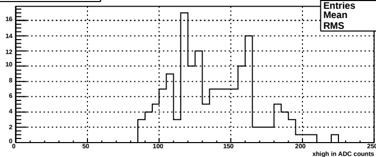
xhigh for bsm dp plane, mod 99
