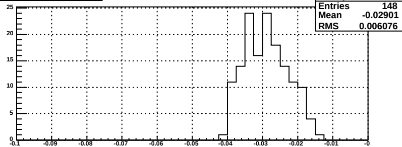
slopes for bsmde plane, mod 99
