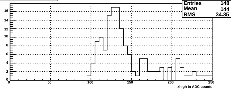
xhigh for bsmde plane, mod 99
