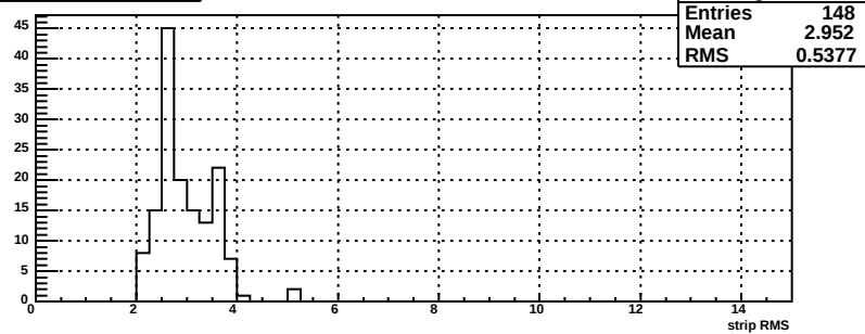
rms for bsmde plane, mod 99
