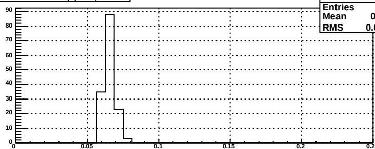
relative errors for bsm dp plane, mod99
