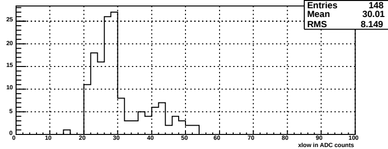
xlow for bsmde plane, mod 99
