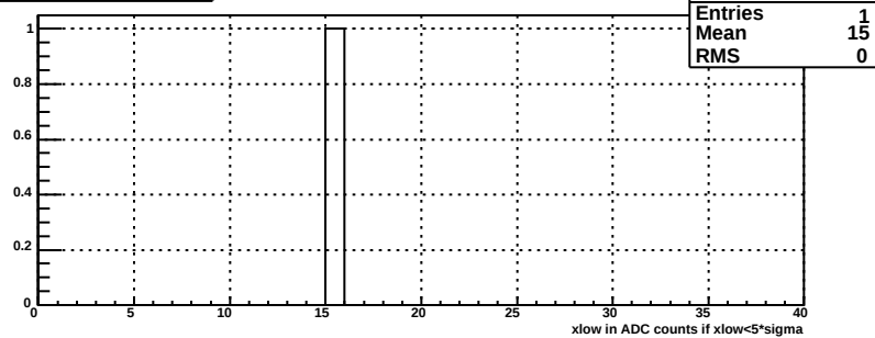
nlow for bsmde plane, mod 99
