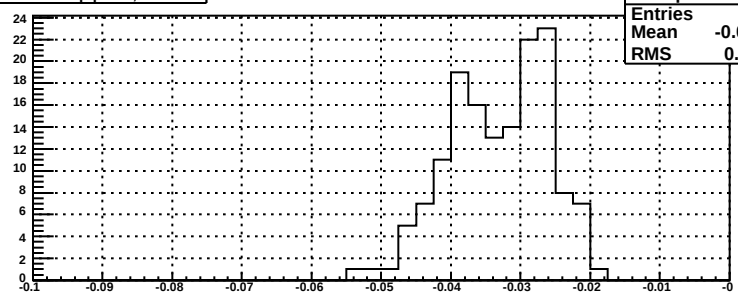
slopes for bsm dp plane, mod 99
