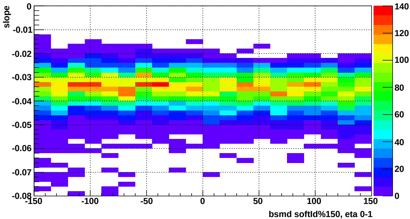
bsmdp slope vs id/15 (excellent modules only)
