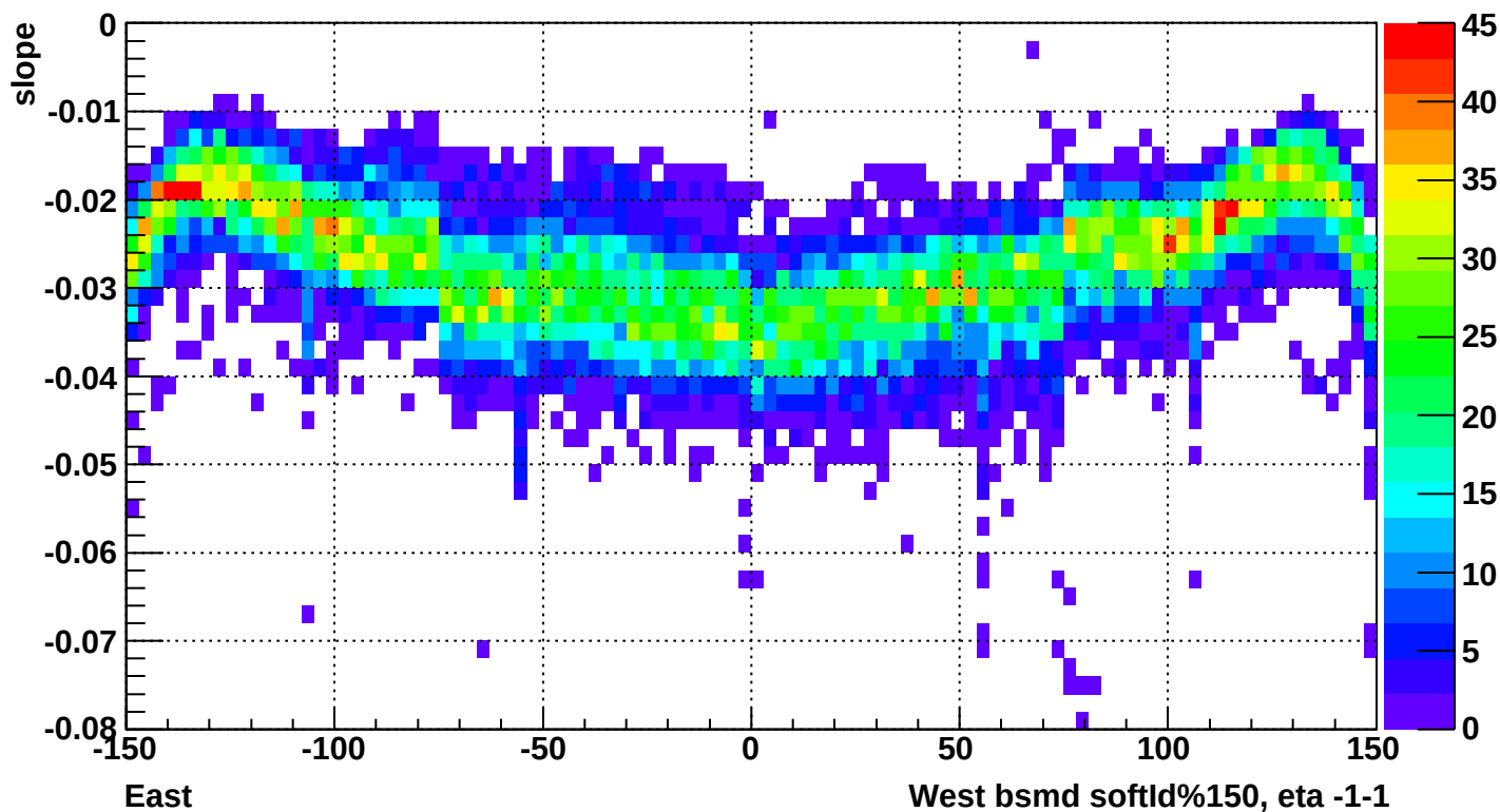
bsmde slope vs. id (1-150) (excellent modules only)
